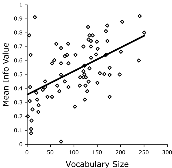
Figure 3: Information value of variation sets in the corpus of Waterfall (2006). The mean information value of the maternal variation sets is most correlated with the size of child’s productive vocabulary ( R^2 = 0.21 ) for \beta = 0.487 . For points with vocabulary size > 25 , the regression is more pronounced ( R^2 = 0.40 ).
