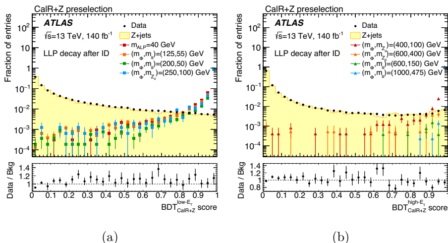
Figure 4. Comparison of the distribution of (a) \text{BDT}_{\text{CalR+Z}}^{\text{low-}E_T} and (b) \text{BDT}_{\text{CalR+Z}}^{\text{high-}E_T} scores between signal events and background, after preselection. In all cases, only signal events with at least one LLP decaying after the ID are shown. The simulated background events are shown only for comparison at the preselection stage, and are not used in the final background estimate.
