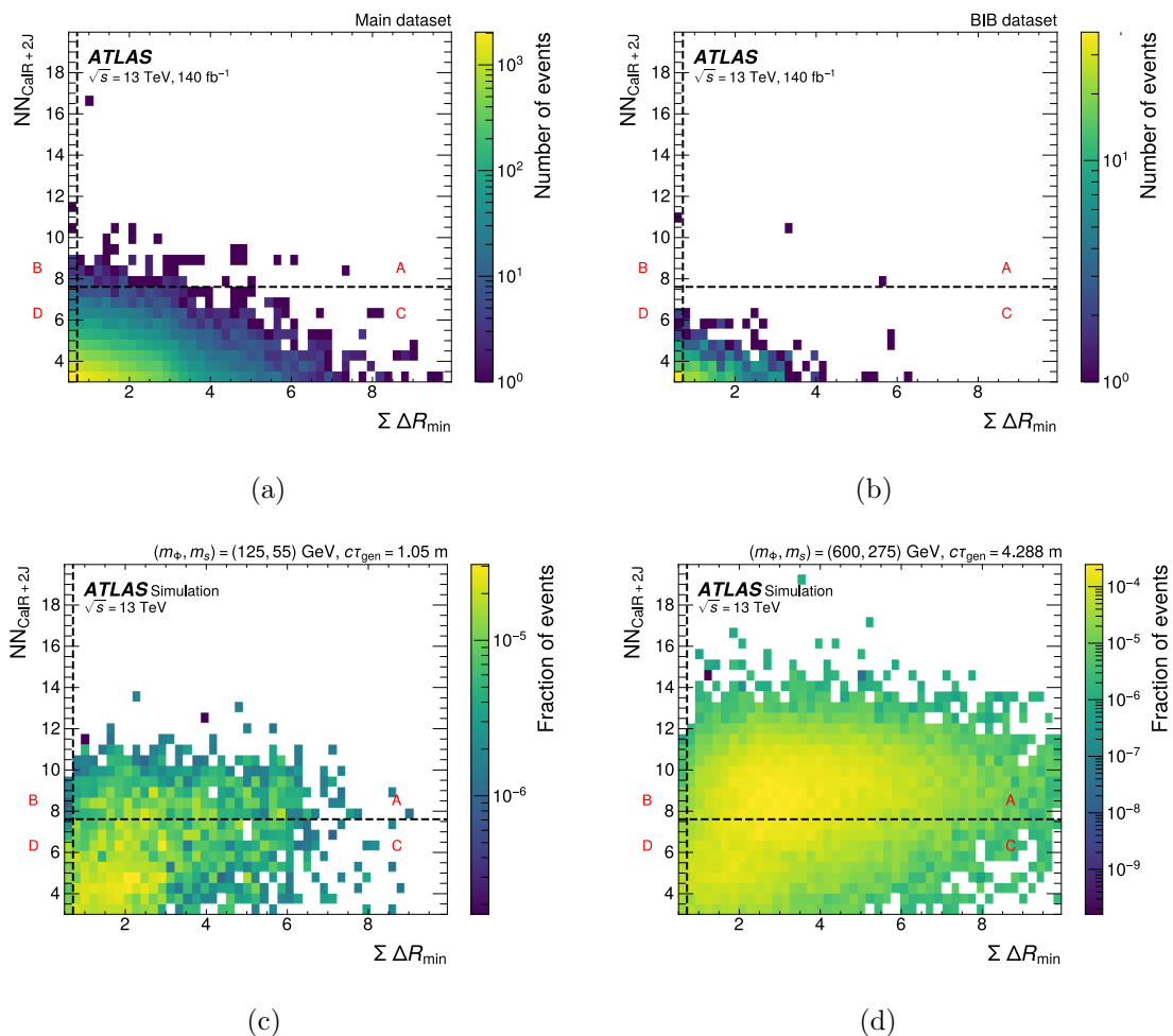
Figure 5. Distribution of events in the two-dimensional plane of NN_{\text{CalR}+2J} vs. \Sigma \Delta R_{\text{min}} in the CalR+2J channel for (a) the main dataset, (b) the BIB datasets, and (c, d) example benchmark signal samples. Final regions A, B, C and D are marked in red.
