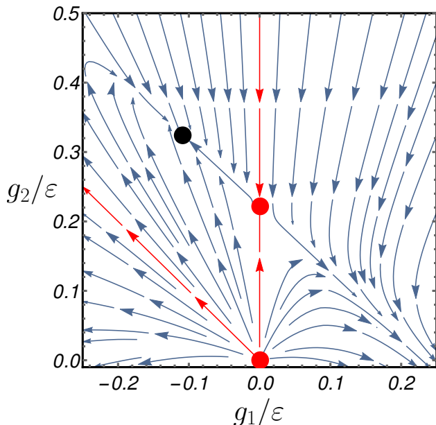
FIG. 2. Global phase diagram of the RG flow described by Eq. (27) for both the FM and SmA-C transitions. The region g_1 > 0 describes a runaway flow signaling a first-order phase transition. The line g_1 = 0 governs the FM transition in the inversion-symmetric system, which is controlled by the IS fixed point. The region 0 < -g_1 < g_2 is controlled by an interacting fixed point (black) and describes the second-order SmA-C transition in a magnetic field. The line -g_1 = g_2 describes the SmA 'critical phase', with the parameters g_1, g_2 flowing to the Sm fixed point (not shown in this figure, see also Fig. 4).
