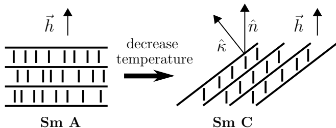
FIG. 3. Schematic representation of the smectic-A to smectic-C transition in a magnetic field, \vec{h} . The transition occurs via tilting of the layers, and is characterized by a nonzero angle between the molecules' director \hat{n} and the smectic layer normal, \hat{k} (see Ref. 20).
