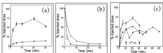
Figure 3. Uptake of 125 I-labeled siRNA–GalNAc conjugate 20 into livers of wild-type mice after IV administration. (a, b) % injected dose (ID) detected as a function of time after 0.5 mg/kg dose (a) in liver with (–▲–) and without (–●–) and (b) in serum with (–△–) and without (–○–) pretreatment with free ligand. (c) % ID in liver after a 0.5 mg/kg single dose (–○–) and after two consecutive 1 mg/kg doses at t = 0 and 10 min (–●–) or t = 0 and 30 min (–▲–). Error bars are standard deviations.
