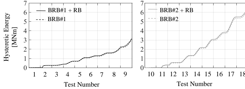
Figure 5: BRB+RB connection and BRB hysteretic energy dissipation.
