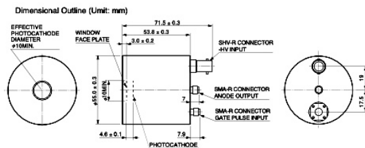
Figure 1. Hamamatsu gateable microchannel plate photomultiplier R5916U-50 Series.
