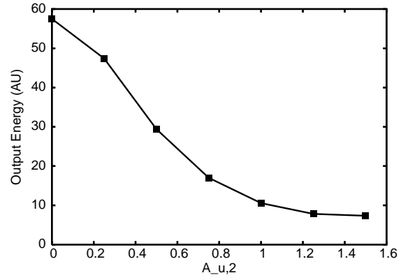
Figure 2: Outgoing radiation energy beyond the undulator exit as a function of a_{u,2} for a biharmonic undulator with \lambda_{u,2} = 3\lambda_{u,1} and a_{u,1} = 1.0 .
