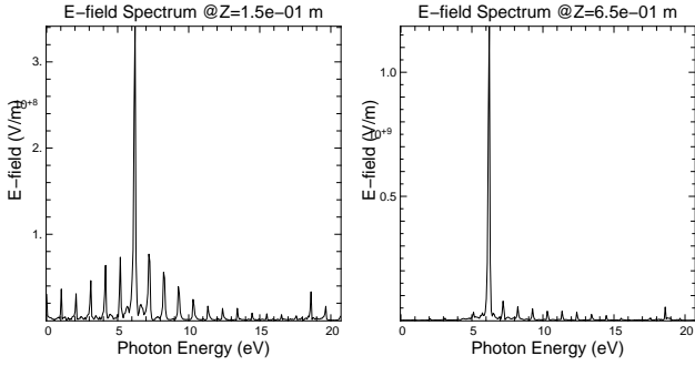
Figure 1: On-axis electric-field spectrum |E(\omega)| at z = 0.15 m (left plot) and z = 0.65 m (right plot) from an electron beam sub-harmonically bunched at \lambda = 1200 nm in an undulator resonantly tuned to \lambda_R = 200 nm ( \hbar\omega = 6.1 eV). In addition to strong sideband emission early in z whose blueward components persist later in z , there is also evident third harmonic emission at 18 eV.
