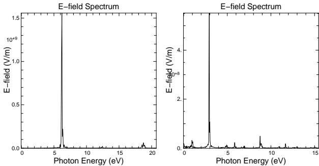
Figure 3: On-axis electric-field spectrum |E(\omega)| from (left) a "normal", single frequency undulator with a_{u,1} = 1.0 and (right) a biharmonic undulator with \lambda_{u,2} = 3\lambda_{u,1} , a_{u,1} = 1.0 and a_{u,2} = 1.5 .
