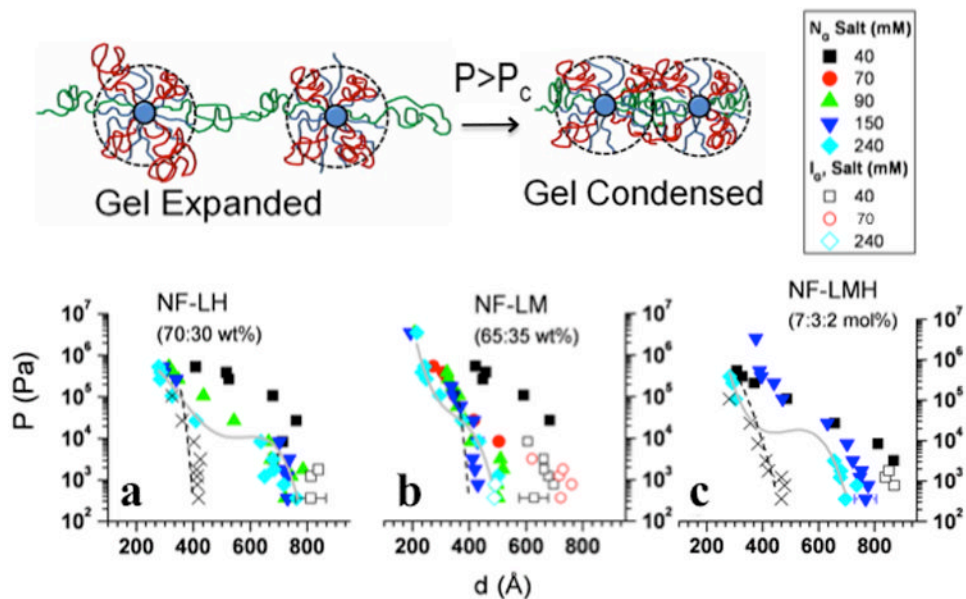
Figure 5. (Top) End view of NF-LH, NF-LMH hydrogels undergoing a transition for P > P_c from an expanded-network to a condensed-network gel state with interpenetrating sidearm polyampholyte chains. (Bottom) Pressure-interfilament distance curves for NF hydrogels obtained using the SAXS-osmotic pressure technique. At ionic strengths 150 mM and 240 mM NF-LH (a) and NF-LMH (c) gels exhibit an expanded-network to condensed-network transition for P > P_c \approx 10^4 Pa, whereas NF-LM gels (b) are in a compressed state for P < P_c and transition to the condensed state for P > P_c . ( N_G = nematic gel; I_G = isotropic gel). At low ionic strengths (40 mM and 70 mM) NF-LM gels are expanded isotropic gels at P < P_c and transition to the condensed-network state at P > P_c . Reprinted in part with permission from [25].
