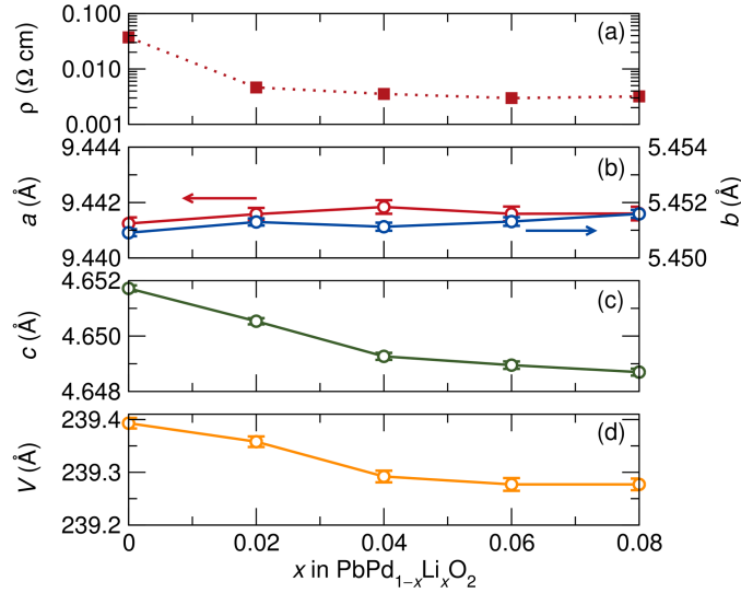
Figure 3: Room temperature resistivity, lattice parameter and unit cell volume changes as a function of Li substitution in \text{PbPdO}_2 . Only the c parameter changes significantly up to 4 mol% Li. The constant values above 4 mol% suggest a solubility limit of Li in the structure. Error bars indicate one standard deviation.
