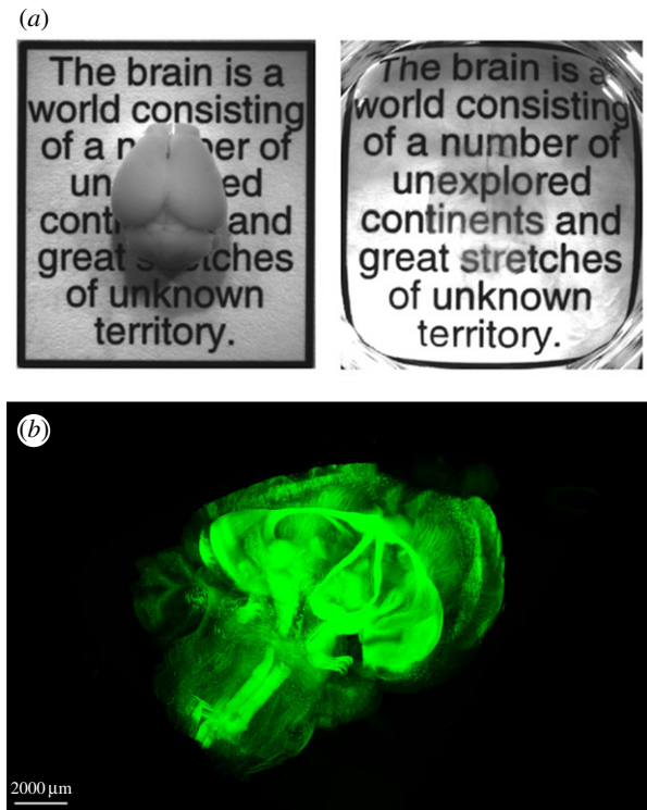
Figure 2. Integrating neuroscience and chemical engineering—CLARITY technique. Images courtesy of the Deisseroth Laboratory, Stanford University. (a) Mouse brain prior to CLARITY transformation (left). Following CLARITY, the brain is rendered transparent while preserving its structural integrity (right). (b) High-resolution fluorescence signals (as well as antibody labels and oligonucleotide probes) pass entirely through intact brains in CLARITY (shown is an adult mouse brain with long-range projections labelled in green with a genetic marker).
