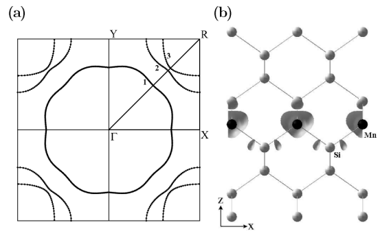
FIG. 4. (a) Calculated two-dimensional Fermi surfaces. (b) Majoritiespin hole charge density in the vicinity of E_F for Mn \delta -doped in Si.
