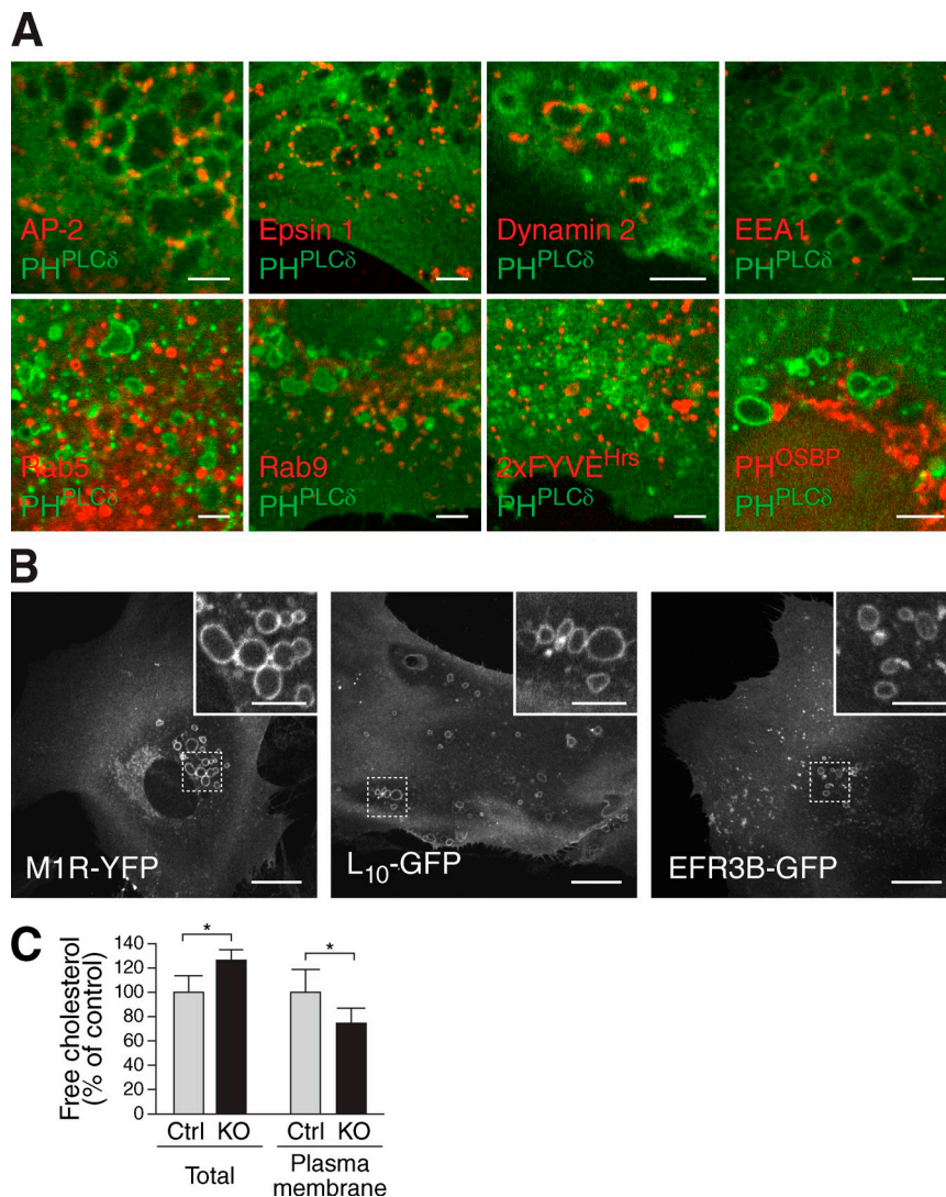
Figure 8. Loss of plasma membrane identity in PI4KIII \alpha KO MEFs. Proteins typically restricted to the plasma membrane are found on intracellular PtdIns(4,5)P 2 -positive vesicles, which are negative for a variety of endosomal and Golgi markers. (A) PtdIns(4,5)P 2 -positive intracellular vesicles, visualized with GFP- or RFP-PH PLC \delta , colocalize with endocytic clathrin machinery components (endogenous AP-2, epsin 1, and dynamin 2–GFP) but not with markers of endosomes (endogenous EEA1, GFP-Rab5, and GFP-Rab9), the endosomal phosphoinositide PtdIns3P (GFP-2xFYVE Hrs ), and Golgi-localized PtdIns4P (GFP-PH OSBP ). For clarity, PH PLC \delta is false colored green, and the second marker is false colored red in all images. (B) Mislocalization of plasma membrane proteins in cells lacking PI4KIII \alpha . PI4KIII \alpha KO MEFs were transfected with M1R-YFP, L 10 -GFP, or EFR3B-GFP and imaged by confocal microscopy. Note the accumulation of all markers in intracellular vesicles highlighted in the inset images. (C) Measurement of total and plasma membrane fraction of free cholesterol in control and PI4KIII \alpha KO MEFs. Total free cholesterol levels were measured by HPLC, after lipid extraction, and normalized to total cellular phospholipid levels. *, P < 0.0001 ( n = 12 for control and KO). Plasma membrane free cholesterol was measured by treatment of cells with 10 mM M \beta CD for 1 min followed by quantification of extracted cholesterol using an enzyme-coupled assay and normalization to total protein content. Error bars indicate standard deviations. *, P < 0.02 ( n = 6 for control and KO). Bars: (A and B, insets) 5 \mu m; (B, full size images) 20 \mu m.
