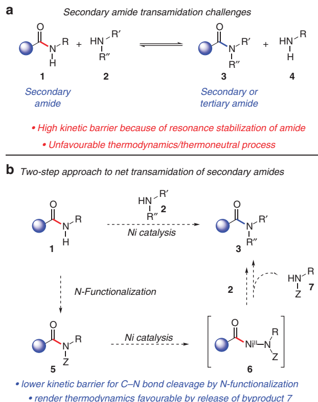
Figure 1 | Development of Ni-catalysed secondary amide transamidation.
