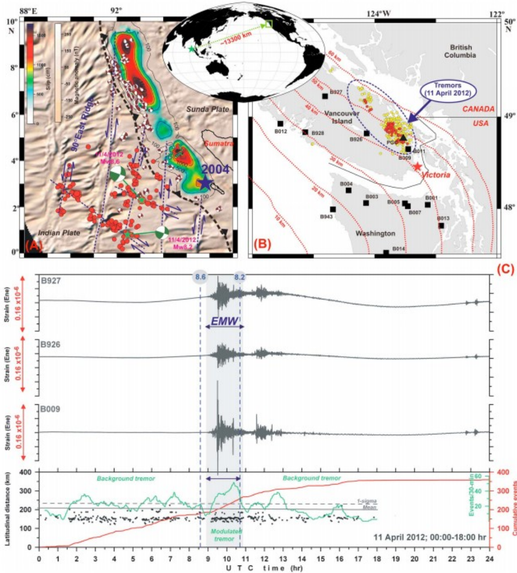
Figure 1. Tectonic tremor activity in the Cascadia subduction zone modulated by the 11 April 2012 East Indian Ocean earthquake. (a) Magnetic anomalies [http://geomag.org/models/wdmam.html] and general tectonics of Sumatra subduction zone and location of the 11 April 2012 East Indian Ocean earthquakes ( M_w 8.6 and M_w 8.2). The 2004 Sumatra-Andaman earthquake rupture in the Sumatra frontal arc [Chlieh et al. , 2007] and its epicenter is also shown. Fracture zones are identified on the basis of swath bathymetry data [Graindorge et al. , 2008]. (b) The yellow filled circles are the catalogued tectonic tremors near Vancouver Island that occurred on the day of the 11 April 2012 East Indian Ocean earthquake. Tremor locations are taken from pnsn.org. The solid squares show the borehole strainmeters and seismometers of the Plate Boundary Observatory (PBO). The solid triangle denotes the broadband station, PGC, operated by the Canadian National Seismograph Network (CNSN). Isodepths of plate interface (at 10 km depth intervals) are also shown by red dashed lines [Houston et al. , 2011]. (c) Temporal variations of shear strain (Ene) at the three nearest PBO borehole stations (B009, B926, and B927) are shown in the upper three panels. The blue dashed lines are the origin times of the two earthquakes. The bottom figure shows the origin time of tremors (black dots) and cumulative number of tremor detections on Vancouver Island (red curve) on 11 April 2012. The rate of tremor activity in 30 min sliding window with 1 min shift is shown by green curve with the mean rate and 1\sigma value of tremor activity during the tremor swarm shown by horizontal solid and dashed lines, respectively. The red filled circles denote the tremors during effective modulation window (EMW) shown by gray shading in Figure 1c.
