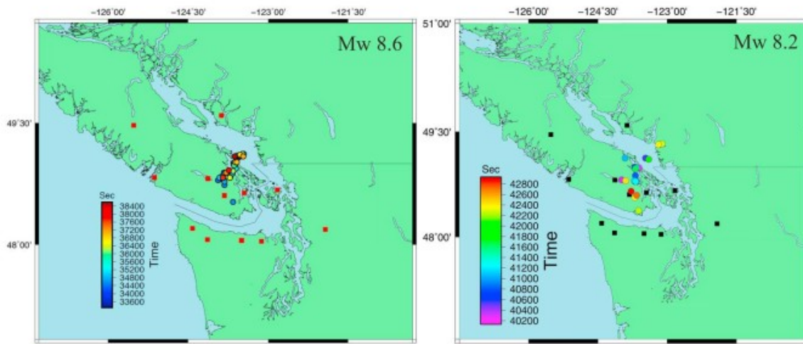
Figure 3. Modulated tremor in Cascadia during M_w 8.6 and M_w 8.2 events. Seismic stations (marked by squares) used to locate modulated tremor (circles colored by time) in Cascadia during M_w 8.6 and 8.2 events, respectively. A spatiotemporal map shows the high-quality tremor locations from time of S wave modulating to Rayleigh wave modulating.
