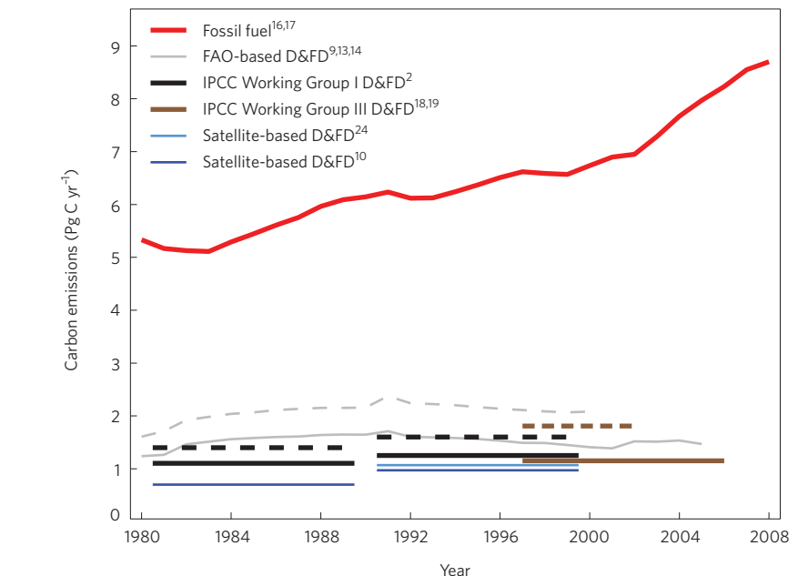
Figure 1 | Carbon emissions from deforestation and forest degradation (D&FD) and fossil fuel emissions for 1980 onwards. Updated datasets and approaches are depicted with a solid line, outdated ones with a dashed line. The often-held assumption that deforestation and forest degradation accounts for 20% of global anthropogenic CO 2 emissions is calculated using the average (dashed black line) of the deforestation surveys from the Food and Agricultural Organization (FAO; dashed grey line) and satellites in the 1990s (dark blue line), compared with average fossil fuel emissions estimates for the 1990s (red). Revised FAO-based emissions estimates (solid grey line) together with increased fossil fuel emissions substantially lower the relative contribution of deforestation and degradation to total anthropogenic emissions to about 12%. Dashed brown line indicates D&FD assessment used in IPCC Working Group III; solid brown line follows the same approach, but is based on updated carbon emissions from tropical forest fires used in this approach. Error bars are not shown, but the uncertainty in the deforestation figures is large, up to 50%. Peatland carbon emissions (0.30 Pg C yr -1 ) are not included in emissions estimates.
