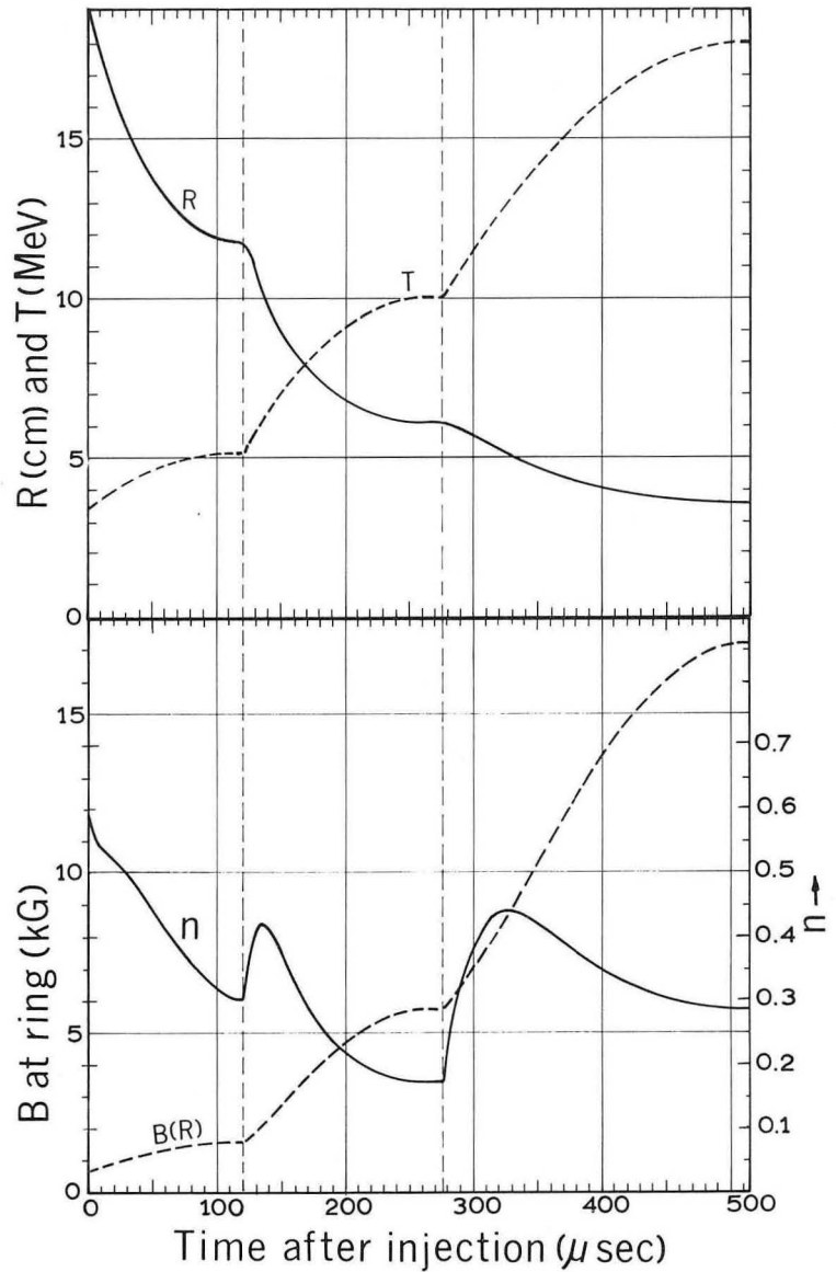
Fig. 3 The major radius ( R ) of the ring, the kinetic energy ( T ) of the electrons, the magnetic field ( B ) at the ring, and the magnetic field index ( n ), as functions of time during the compression of the ring in a typical cycle.
