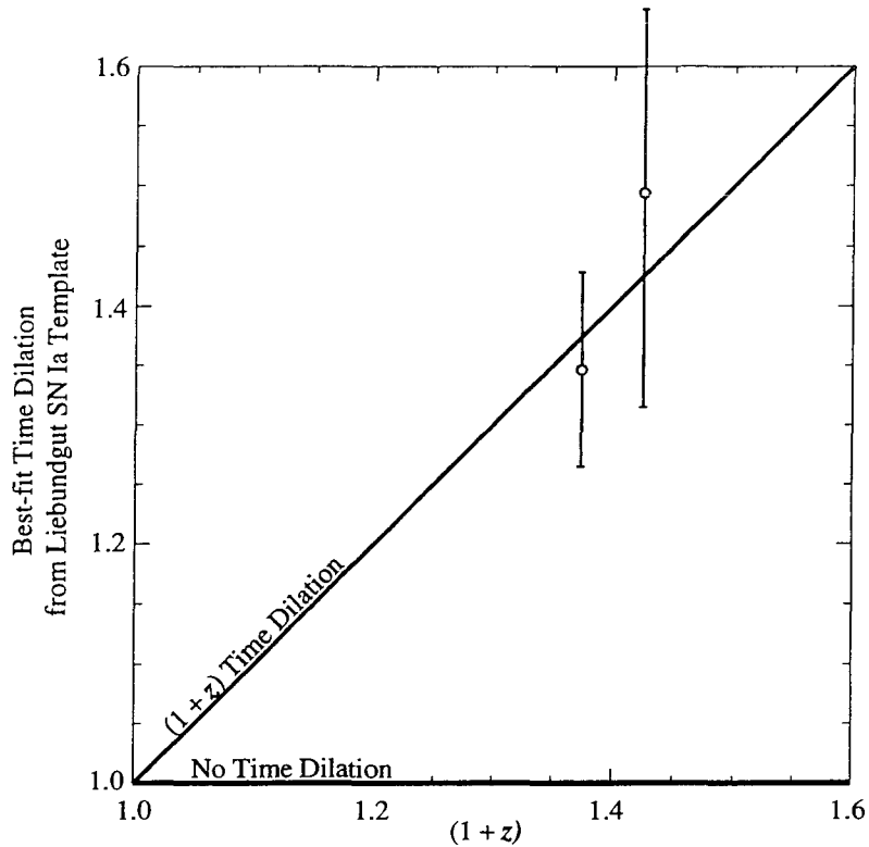
Figure 3. A plot of d/s for two of our SNe, SN94H and SN94G for which the stretch, s , was deduced from the SNe colors.
