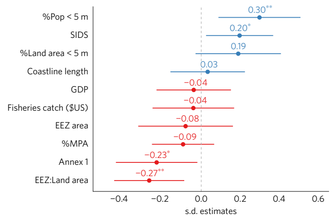
Figure 4 | Ability of different explanatory variables to explain variance in NDC marine focus. Standardized coefficients from the multiple linear regression with Marine Focus Factor (MFF) as the dependent variable. Variables with positive (blue) and negative (red) impacts on MFF shown, with bars indicating two standard deviations in the error estimate. Asterisks denote statistically significant variables (* p < 0.05 , ** p < 0.01 ). Explanatory variables tested were: percentage of the population living in areas less than 5 m above sea level (%Pop < 5 m), whether the country was a SIDS, percentage of land area that was less than 5 m above sea level (%Land Area < 5 m), the coastline length (m), the GDP, the domestic fisheries landing value (Fisheries Catch ($US)), the total EEZ Area, the percentage of the marine territory that was protected (%MPA), whether the country was an Annex 1 Party, and the ratio of EEZ to land area (EEZ:Land Area).
