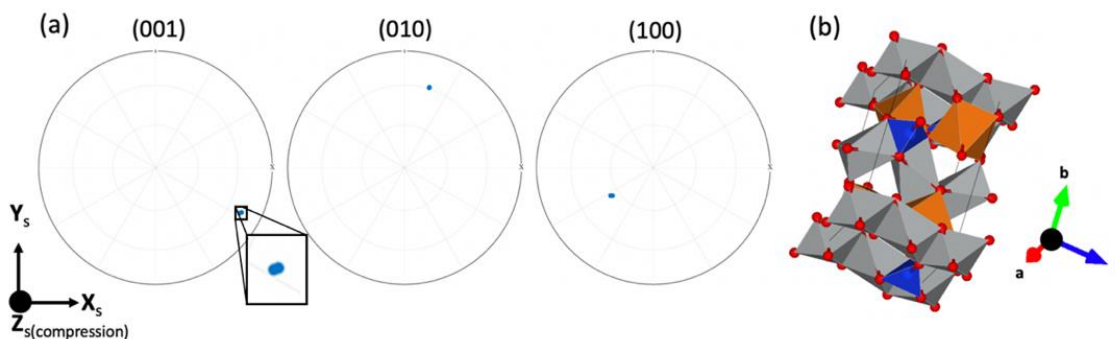
Figure 6. (a) Equal area upper hemisphere pole figures of the crystallographic axes in both identified olivine orientations depicted by blue dots. Notice the tight two spot cluster indicating two unique orientations compared to Figure 5a–c. The X_s direction in the sample frame is to the right with Z_s coincident with the DAC compression direction out of the page (depicted in the lower left). (b) A polyhedral rendering of the olivine structure in the identified orientation with direct lattice vectors (a–c) in bottom right.
