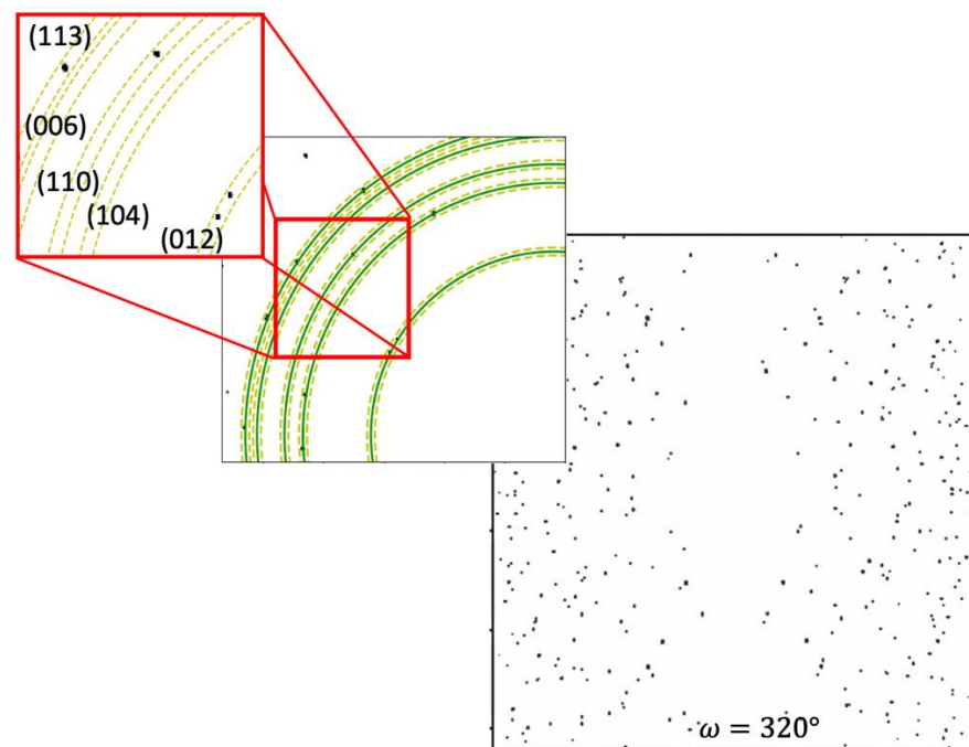
Figure 3. (Right) Aggregate diffraction image of NIST ruby sphere collected over 320^\circ [ -100, 220^\circ ] in \omega (Middle) Reference 2\theta values (green lines) for selected G_{hkl} with initial 2\theta tolerances (dashed yellow) applied globally to the image set. (Top Left) Measured intensities falling within the specified tolerances are used for orientation space segmentation and initial candidate grain identification. Here, the tolerances for (113), (006), (110), (104), and (012) are shown with visualized Bragg reflections for (113), (110), (104), and (012) in these azimuthal segments (Top Left, Middle).
