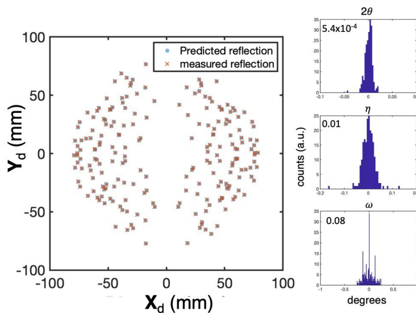
Figure 4. (Left) Comparison of predicted (blue circle) to measured (red x) spot locations for the NIST ruby sphere used for 3D detector calibration. (Right) Histograms showing deviation of measured diffraction spot locations compared to reference lattice predictions on the 2D detector face in the angular coordinate system (2\theta, \eta, \omega) described in Figure 1. Average deviation shown in top left corner.
