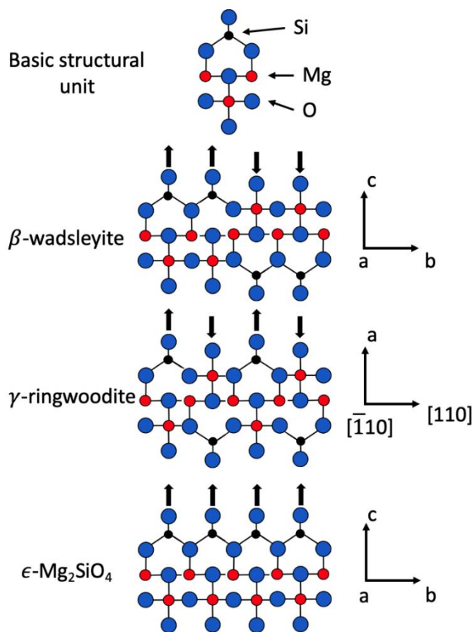
Figure 9. Crystal structures of the Mg 2 SiO 4 spineloids ( \beta , \epsilon ) and spinel ( \gamma ) modified from [53] showing the relation of each crystal structure based on the orientation of the basic unit structure (Top).
