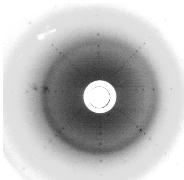
FIG. 1. X-ray Laue diffraction image of our \text{PrB}_4 sample. The platelet plane was oriented perpendicularly to the x-ray beam.
