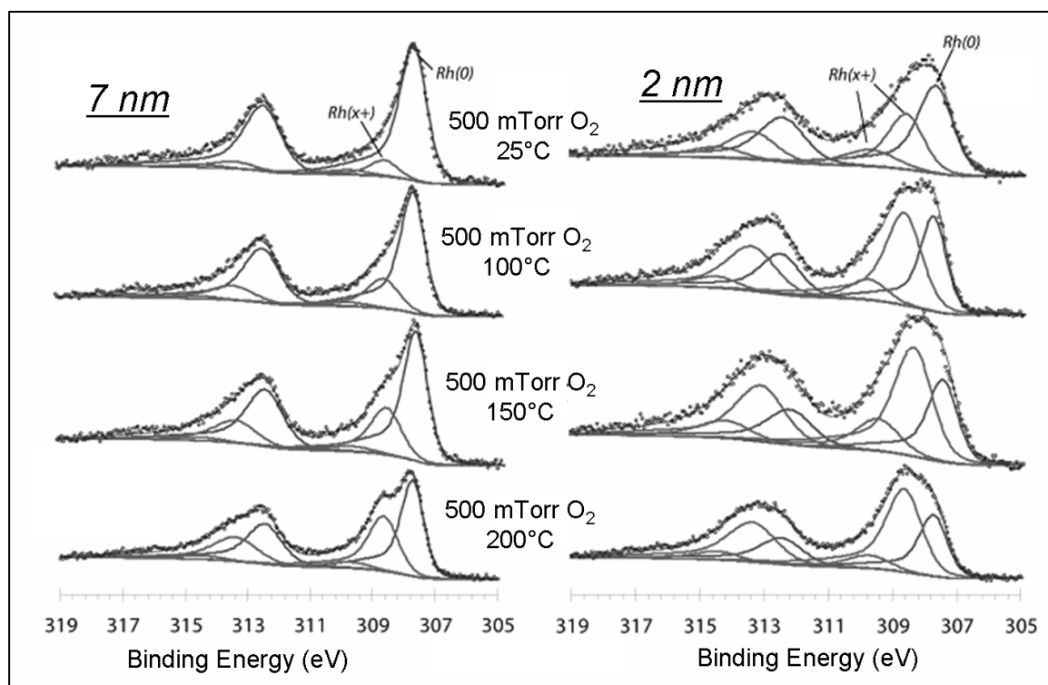
Figure 6.5 Rh 3d spectra of 7 (left) and 2 (right) nm particles at in the presence of 500 mTorr O 2 . As the temperature increases, the Rh nanoparticle surface becomes in increasingly oxidized with the 2 nm particles oxidizing at a lower temperature.
