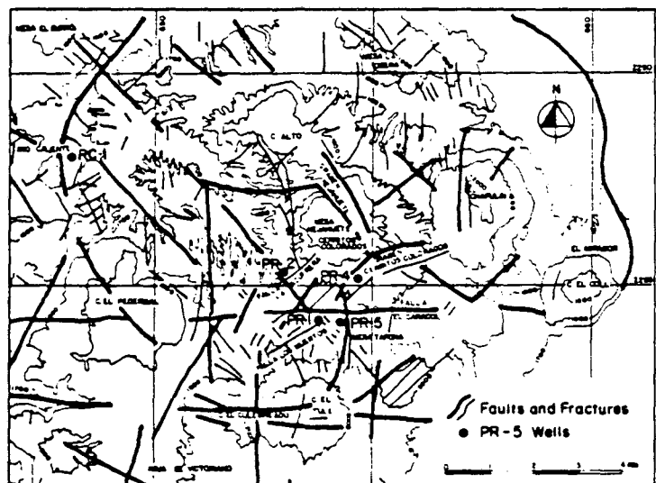
Figure 2. Structural map of the La Primavera field showing the location of the exploration wells.
