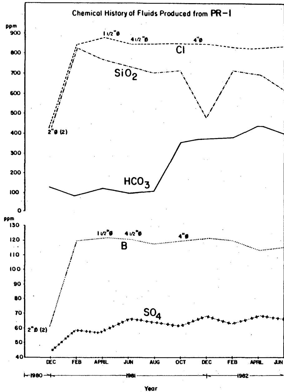
Figure 13. Well PR-1. Chemical history of produced fluids.
