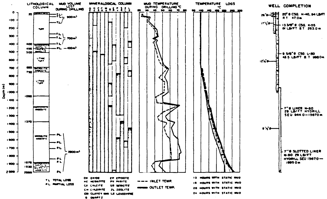
Figure 6. Well PR-2. Drilling and completion data.
