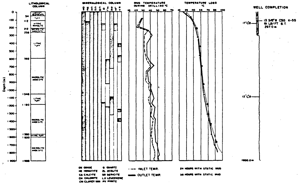
Figure 5. Well RC-1. Drilling and completion data.
