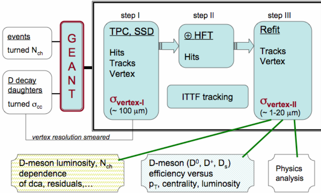
Figure 16: Simulation block flow diagram. Only small modifications were needed to optimize the STAR reconstruction software for use with the HFT.
