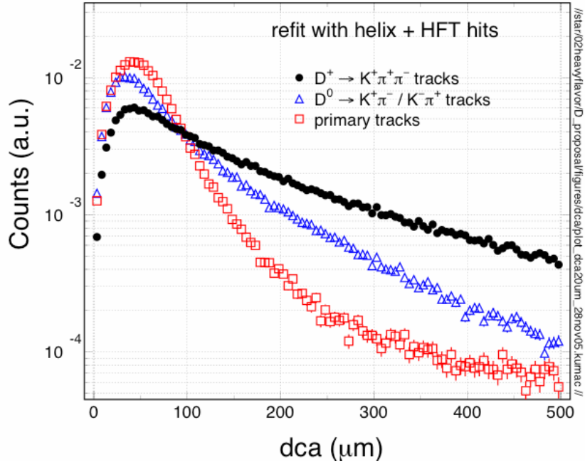
Figure 23: The distance of closest approach (dca) distributions for D^0 (triangles) and D^+ (circles). The results of the dca distribution for primary tracks are shown in squares.
