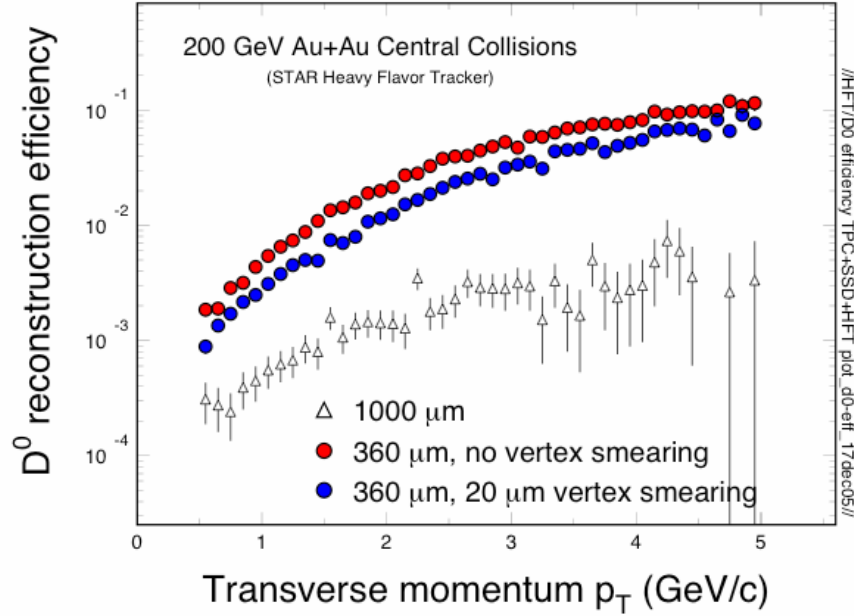
Figure 27: The absolute yield of D^0 into the TPC + SSD + HFT divided by the input D^0 yield. For comparison, a simulation with thick Si detectors that are similar to the wafers used in the ALICE vertex detector is also shown (1000 \mu\text{m} effective silicon thickness).
