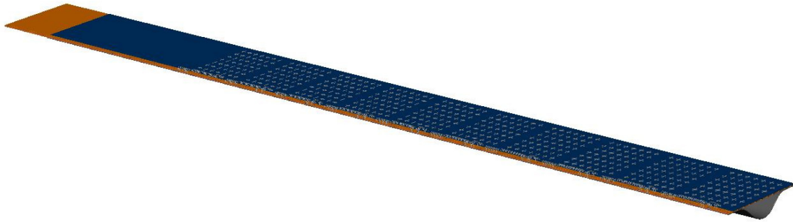
Figure 54: Ladder assembly. The current ladder is composed of a row of 10 thinned APS detectors on top of a matching row of thinned readout chips and a three-layer aluminum Kapton cable. The silicon cable structure is bonded to a carbon composite “v”, closing the beam to make a rigid structure.
