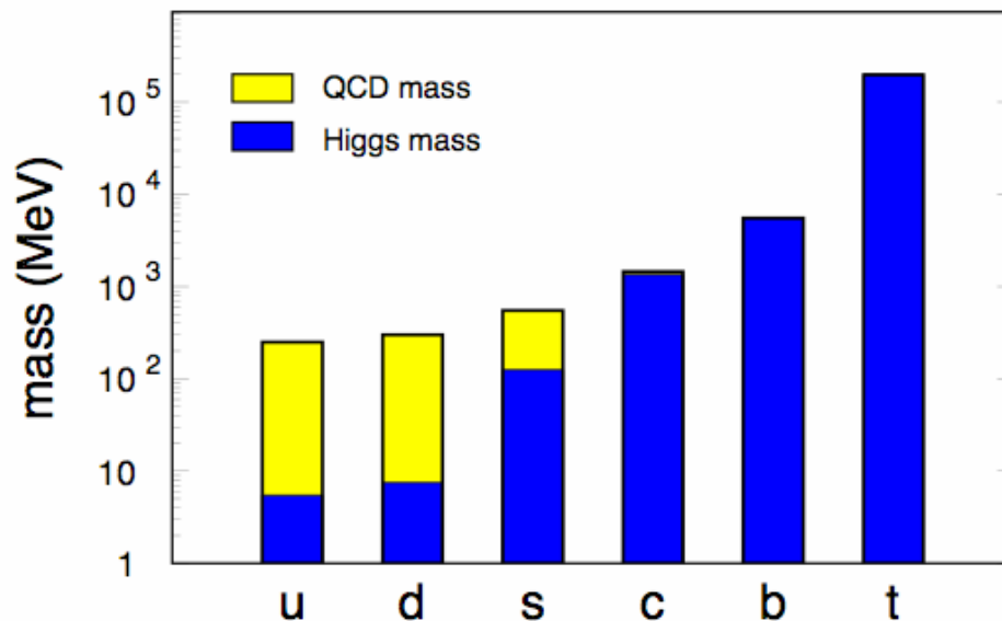
Figure 1: Masses of the six quark flavors. The current and additional QCD masses are shown by blue- and yellow-boxes, respectively. The figure is adapted from Ref. [12].
