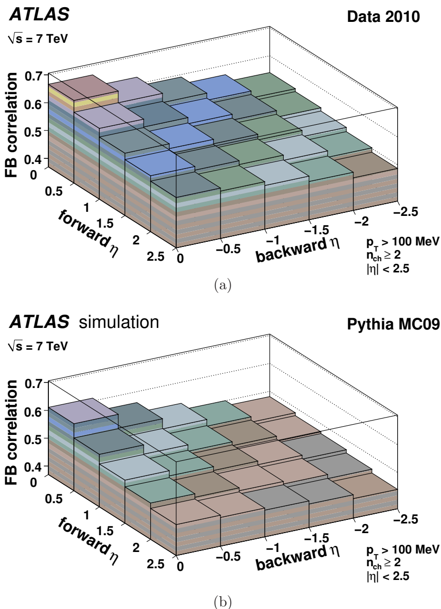
Figure 2. Multiplicity correlation at 7 TeV in a matrix of forward/backward \eta -intervals for |\eta| < 2.5 , for events with at least two charged particles with p_T > 100 \text{ MeV} and |\eta| < 2.5 . (a) data; (b) PYTHIA 6 MC09 tune. The statistical uncertainties are of the order of \pm 0.001 .
