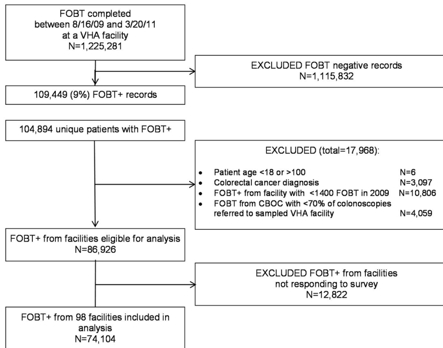
Figure 1. Subject Flowchart
