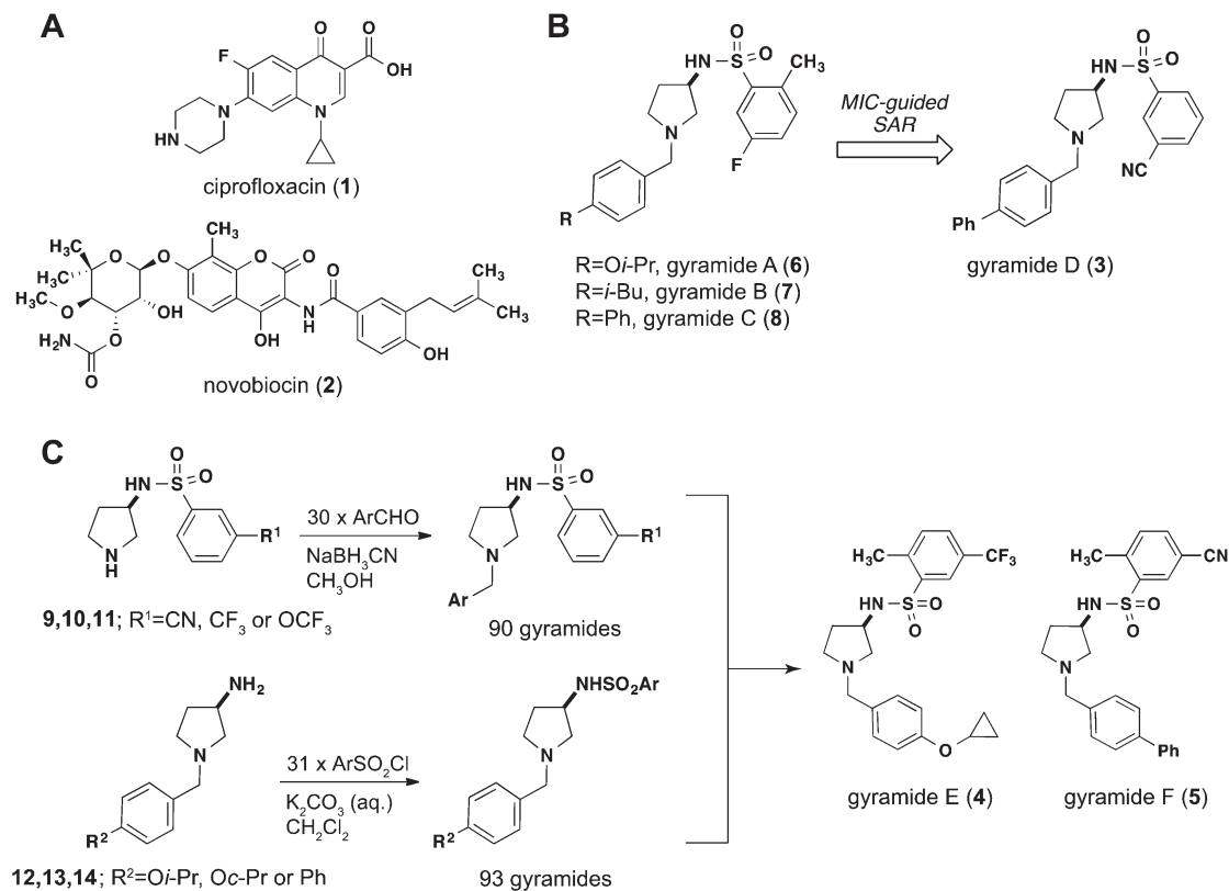
Fig. 1 A) The chemical structures of ciprofloxacin (1) and novobiocin (2). B) 3 was created from a MIC-guided SAR study of 6–8 . 3 has activity against wild-type E. coli and was used as a lead structure for further analog design and synthesis. C) Design of a chemical library of 183 gyramide analogs. Two reactions were performed with 30 aldehydes (and 3 arylsulfonamides) and 31 sulfonyl chlorides (and 3 arylamines) to create 183 gyramide analogs.
