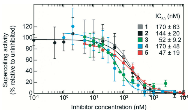
Fig. 2 Dose-response curves for DNA gyrase-dependent supercoiling activity in the presence of 1, 2, and 3–5. We performed DNA supercoiling reactions with E. coli DNA gyrase, relaxed pUC19 plasmid substrate, and various concentrations of 1, 2 and 3–5. Reactions were run for 30 min and the DNA was separated on a 0.8% (w/v) agarose gel for 3 h. We labeled the DNA by immersing the gel in a solution of 0.5 mg mL -1 ethidium bromide for 1 h. The fluorescence intensity of the supercoiled DNA band was normalized to the DMSO solvent control and plotted for each concentration of compound tested. See the Material and methods section for experimental details. Each reaction was performed in triplicate. Error bars indicate the standard deviation.
