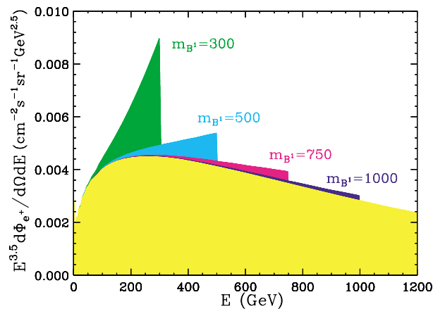
FIG. 2 (color online). Predicted positron signals above background (light shaded area, yellow) as a function of positron energy for m_{B^1} = m_{e_L^1} = m_{e_R^1} = 300, 500, 750, and 1000 GeV.
