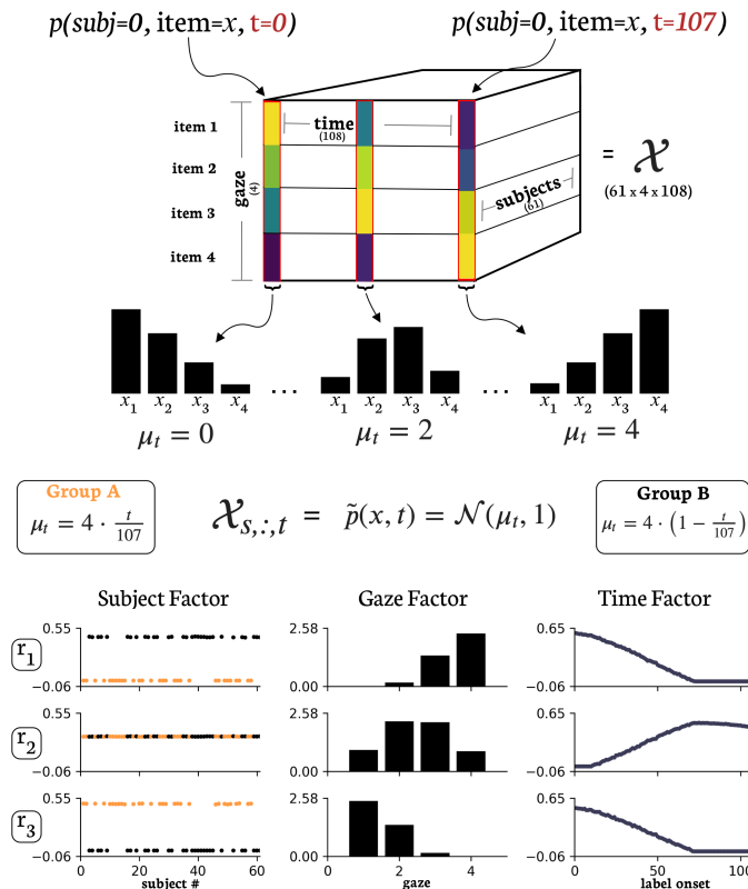
Figure 3: We compute an R = 3 decomposition on synthetic gaze distributions and plot the resulting factors.
