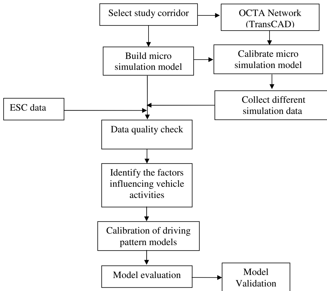
Figure 1 Methodology overview
