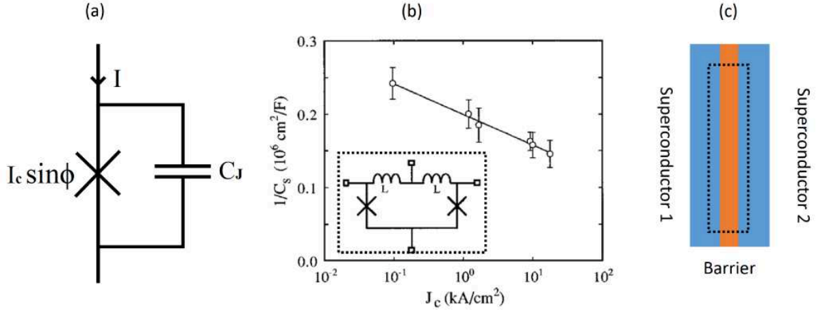
Figure 2.1: (a) Equivalent circuit model of a Josephson junction. Nonlinear inductor is connected parallelly with a capacitor. (b) Specific capacitance of Nb/AIO x /Nb Josephson junctions. [15] Inset in dashed box is the circuit used in the experiment. (c) Two wide superconductors (blue) are connected with a long barrier (orange). The integrated loop along the dashed line can be modeled as the circuit in the inset of (b).
