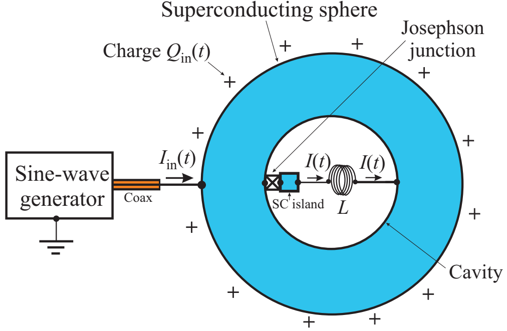
Figure 2.5: In the spherical superconducting (SC) shell, the SC artificial atom is formed with the hollow cavity and a superconducting wire on the horizontal axis. A SC island is connected to the cavity with a SC wire on one end and via a large Josephson junction on the other end. The effective inductance between the wire and cavity can be enhanced by increasing the number of switchbacks depicted as a solenoid. The spherical SC shell is made thick enough to prevent magnetic flux penetration into interior.
