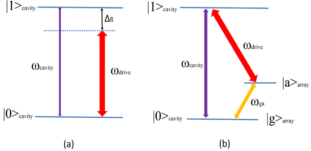
Figure 4.12: The three-wave mixing transition diagram of cooling process. \omega_{drive} is the frequency of driving signal. \omega_{cavity} is the resonant frequency of cooling cavity. \Delta_B = \omega_d - \omega_c is the detuning. Here it shows red-detune. |n\rangle_{cavity} is the photon state of cavity, while, in (b), |g\rangle_{array} |a\rangle_{array} are ground state and one of the excited state of the array, whose energy separation is \omega_{ga} .
