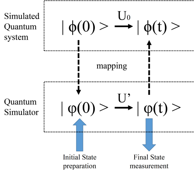
Figure 4.1: A quantum system with state \phi and evolution U_0 is mapped to a quantum simulator with state \varphi and simulative evolution U' . Initial state preparation, simulating evolution operator, and final state measurement are the fundamental three steps of doing quantum simulation. [6]
