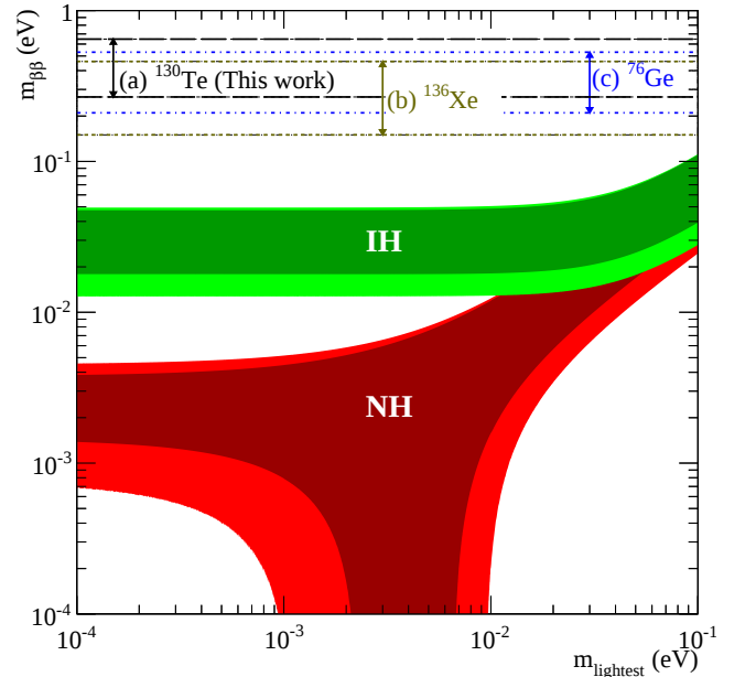
FIG. 15. Plot of the allowed regions for m_{\beta\beta} as a function of the lightest neutrino mass, m_{\text{lightest}} , assuming the light Majorana neutrino exchange model of 0\nu\beta\beta decay. The exclusion bands represent 90% C.L., with the vertical width coming from the uncertainty in the NME. The exclusion from ^{76}\text{Ge} is from [8]. The exclusion from ^{136}\text{Xe} is the combined limits from [9, 10]. The exclusion from ^{130}\text{Te} is the result of this paper. The bounds on m_{\text{lightest}} are from [44]. Figure from [11].
