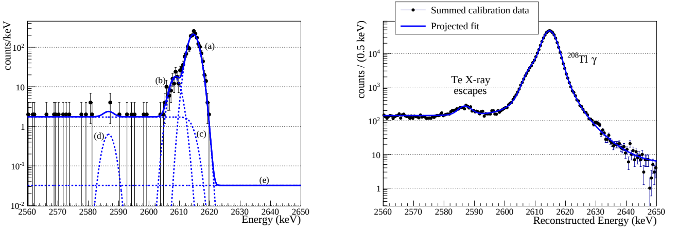
FIG. 8. Left : Best-fit model to the calibration 2615 keV peak for a single bolometer-dataset. The solid line shows the full summed model, and the dashed lines show the individual components: (a) the primary peak of the detector response; (b) the secondary peak of the detector response; (c) the smeared step-function; (d) the X-ray escape peak; (e) flat background. Right : The calibration spectrum summed over all BoDs pairs, with the summed best-fit model. Figure adapted from [11].
