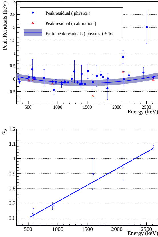
FIG. 9. Top : Residuals of the best-fit reconstructed peak energy and expected peak energy (fit - expected) for the physics data (blue circles) and calibration data (red triangles). The blue curve and shaded band are the fit to the physics peak residuals \Delta\mu(E) and the 1\sigma uncertainty band. Figure adapted from [11]. Bottom : Best-fit resolution scaling parameter, \alpha\sigma , for a few of the peaks in the physics spectrum, as well as the best-fit interpolation.
