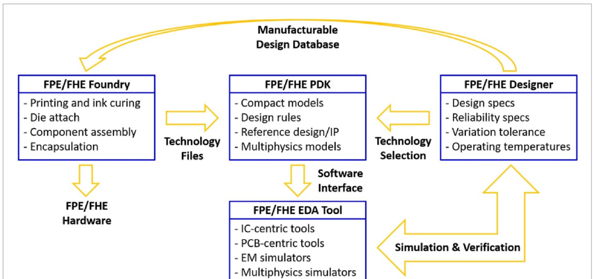
Figure 28. The FPE/FHE design-manufacture ecosystem enabled by the PDK. The PDK includes the latest technology files that represent the manufacturing capability and target performance in the forms of design rules and compact models. The PDK could also include multi-physics models for multi-physics simulation under various thermal or bending conditions, as well as design intellectual property (IP) blocks or reference designs for FPE/FHE designers. The PDK also needs software interfaces for IC-centric or PCB-centric EDA tools in order to perform simulation and physical design verification against the design rules. The designers can also use electromagnetics (EM) or multi-physics simulators with the PDK for radio-frequency (RF) or bending use cases.
