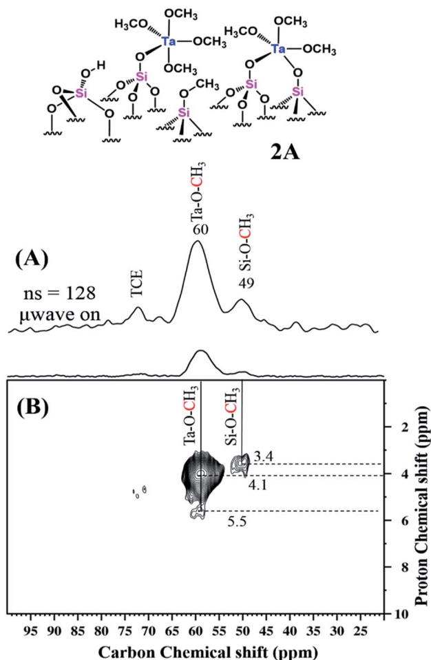
Fig. 7 Schematic representation of 2A followed by (A) 13 C CP MAS with echo DNP SENS spectra (100 K, 400 MHz/263 GHz gyrotron) of 2A impregnated with 16 mM TEKPOL in TCE solution. The spectra were recorded using 128 scans under microwave irradiation, recycle delay of 3 s, contact time of 3 ms, and MAS frequency at 8 kHz (B) 2D 1 H- 13 C HETCOR DNP SENS spectrum with an echo of 2A acquired with 2048 scans per t_1 increment, 96 individual increments and 0.2 ms contact time. During t_1 , e-DUMBO-1 homonuclear 1 H decoupling was applied, and proton chemical shifts were corrected by applying a scaling factor of 0.57 (Table S1 (ESI † )).
