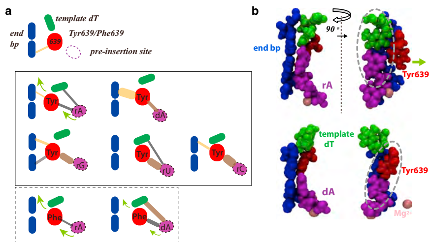
FIGURE 6 The Tyr 639 -assisted nucleotide selection mechanism in T7 RNAP elongation. ( a ) Schematics show how Tyr 639 senses the cognate and noncognate NTPs at preinsertion to allow selective gating during NTP insertion. The four key elements are shown in different colors: (red) residue 639; (blue) end bp of the DNA-RNA hybrid; (magenta) preinsertion NTP; and (green) template DNA nt. Lines linking the elements indicate the nonbonded associations within each pair: (light orange) vdW-dominated; (brown) electrostatic-dominated; (gray) combined; (round head) attraction, i.e., no significant repulsion detected; (thin) weak interaction; (thick) strong interaction. Note that very weak interaction with a strength <1.2 kcal/mol is not shown. The first row shows the posttranslocation configuration. The window (solid line) in the middle shows the preinsertion configurations in the WT, with the cognate rA or noncognate dA/rG/rU/rC bound at the preinsertion
