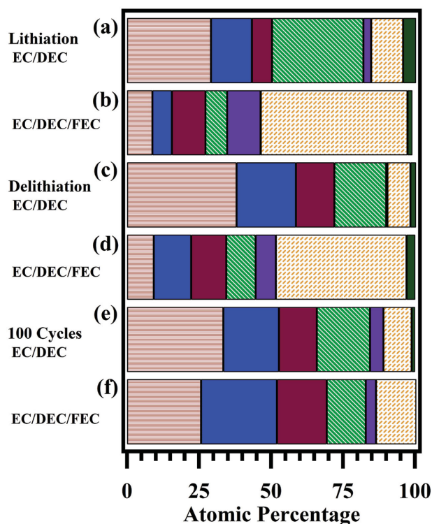
Figure 8. Relative composition of the SEI at Si NPs after a,b) first lithiation, c,d) first delithiation, and e, f) 100 cycles in the delithiated state.
