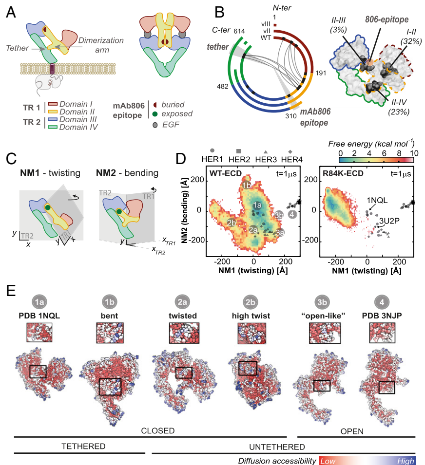
Fig. 1. ENM and MD of tethered ECD predict that N-TR1 twisting renders the 806-epitope accessible in I-II mutants. (A) Scheme of known conformations: the closed tethered ECD (Left), which is inactive, and the active untethered ligand-bound dimer (Right). In both, the 806-epitope is buried. (B) Pattern of missense clusters (black bands) and deletions (EGFRvIII, EGFRvII) along the ECD sequence. Gray arcs indicate C_{\alpha,op} < 10\text{Å} (Left). 3D structure of the tethered ECD (1NQL) with interface clusters in dark (Right). Dashed N-TR1 fragment next to the 806-epitope is deleted in EGFRvIII. I-II interface mutations have the highest clustering (SI Appendix, Fig. S1B). (C) ENM analysis predicts large-scale twisting and bending TR motions (NMs) potentially sensitive to I-II mutations (SI Appendix, Fig. S1 D and E). Note that both NMs expose the 806-epitope, which acts as a molecular hinge, but twisting also releases the dimerization arm. (D) Free-energy landscape from 1- \mu\text{s} MD for clustered I-II (R84K) versus WT-EGFR, shown as projections onto NM1/NM2 together with the HER Family X-ray ensemble (black dots), reveals a highly flexible WT-ECD sampling multiple minima. The reference structure for MD frame and X-ray alignment was 1NQL (state 1a, origin), used for simulation. The WT trajectory shown (Left) departed from 1NQL to sample bent conformations (state 1b) and then visit a low-twist area with tether-truncated structures (state 2a, 3U2P) where untethering happens ( >700\text{ ns} ), followed by further twisting to maximally expose the 806-epitope (state 2b). For R84K (Right), untethering occurs early in the simulation ( >50\text{ ns} ), quickly proceeding to the twisted 806-accessible states energy minima (2a and 2b) and staying there for the remaining time. None of the ECD simulations opens in solution (states 3b and 4). (E) Diffusion accessibility of X-ray and MD conformations: the 806-epitope is maximally accessible in twisted (states 2a and 2b) and bent (1b) MD intermediates. An “open-like” conformation (state 3b) with low accessibility is observed in membranes (SI Appendix, Fig. S3B). The fully open (4) and closed (1a) X-ray structures have an occluded epitope (see SI Appendix, Figs. S2–S4).
