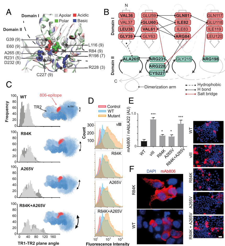
Fig. 3. Increased interfacial flexibility in I-II mutants enhances N-TR1 repositioning as detected by mAb806 binding in HEK293 cells. (A) I-II interface of tethered ECD (1NQL), with protein backbone as cartoon and mutated residues as van der Waals spheres; Consurf score is in parenthesis (variable = 1, conserved = 9). (B) I-II interdomain bonds in MD from 1NQL; note that conserved mutated residues (bold) are interconnected by electrostatic and hydrophobic interactions. (C) MD trajectories of WT-ECD and I-II mutants: TR planes angle distribution for the ECD in solution (100 ns, n = 3 , dark gray) and in constructs with the TM domain (350 ns, n = 3 , light gray) (Left); TR2-alignment of ECD MD frames to show N-TR1 oscillations (50 ns, n = 1 ) versus the 806-epitope (red) (Right). The stable WT angle ( \sim 40^\circ ) occludes the 806-epitope, while N-TR1 oscillations in the double mutant expose it at higher TR angles ( \sim 80^\circ ). (D) FACS binding of mAb806 to HEK293 cells overexpressing WT or I-II mutant EGFR: representative overlays of the fluorescence signal for mAb806-stained cells; mAb806 binds both WT (blue) and mutants (orange) but not control HEK293 cells (red). The right shift of the mean peak in mutants indicates high 806-antigen surface expression, maximal for positive control EGFRvIII and R84K+A265V. (E) Mean fluorescence intensity normalized to total EGFR surface expression (mAbLA22) ( n = 5 ). The double mutant, expected to further disrupt the I-II interface, raises mAb806 binding near to EGFRvIII level. *P \leq 0.05 and ***P \leq 0.001 . (F) Immunocytochemistry of cells expressing WT or mutant EGFR, stained with mAb806 (red) and nuclear marker DAPI (blue), shows enriched localization of 806-antigen to the membrane (see SI Appendix, Fig. S5 ).
