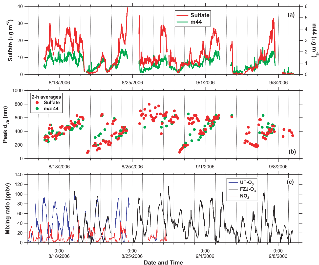
Figure 10. Time series of (a) mass concentrations of \text{SO}_4^{2-} (red) and m44 (green), (b) peak diameters of \text{SO}_4^{2-} (red) and m44 (green), and (c) mixing ratios of UT- \text{O}_3 (blue), FZJ- \text{O}_3 (black), and \text{NO}_2 (red).
