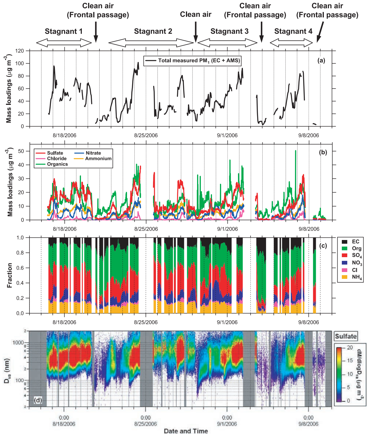
Figure 7. Time series of (a) the mass concentrations of total measured PM_1 aerosol (= EC + OM + SO_4^{2-} + NO_3^- + Cl^- + NH_4^+ ), (b) individual aerosol species measured by the AMS, and (c) fractional contribution of each component to the total measured PM_1 mass. (d) Image plot of size distribution of SO_4^{2-} . The data were smoothed by running mean (boxcar function, 30-min width). The white areas indicate that the signals were lower than noise levels. The noise level was defined as 2 times the standard deviation of the signals at the particle time-of-flight (P-ToF) range of < 1.5 and > 7 ms, where no particle was expected. The gray areas indicate that data were not obtained.
