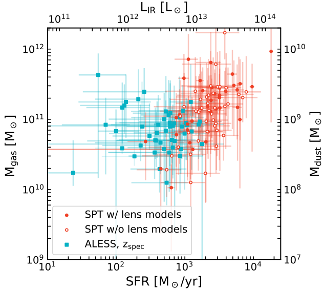
Figure 12. Gas mass versus SFR for the demagnified SPT-selected sources and the ALESS sample. Though the SPT-selected sources have comparable amounts of gas mass to the ALESS sample, the SPT sources also experience higher star formation rates.
