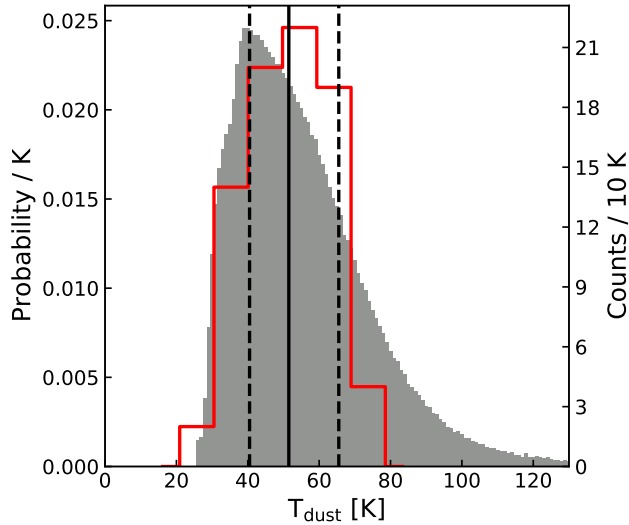
Figure 5. The probability distribution of the dust temperature for all sources in the SPT-DSFG sample. Though this probability distribution peaks at 40 K, the distribution is skewed towards warmer sources. The median of this distribution is at 52.4 K (solid line) and the inner quartiles of the distribution are given by the dashed lines. The adopted median for each fitted T_{\text{dust}} (Tab. F.1) is shown for comparison in red , and is described by the right axis.
