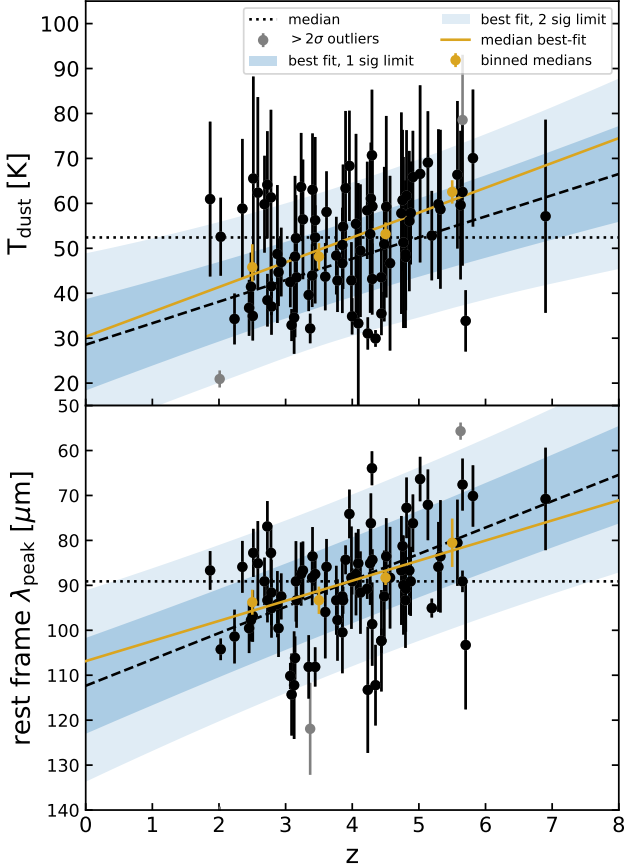
Figure 11. Top: Fitting the dust temperature distribution ( blue ) yields a non-zero linear slope. However, taking into account the intrinsic scatter weakens the significance of such a slope, as reflected in the confidence intervals shown. Outliers ( >2\sigma ) are shown in grey, and removing them does not appreciably change the fitted slope. Binning the dust temperatures with bin widths z=1 also yields a linear dependence ( yellow ). Bottom: Peak wavelength ( \lambda_{\text{peak}} ) versus redshift. The wide sampling of the SED makes the \lambda_{\text{peak}} constraint insensitive to the SED fitting procedure. The same analysis was repeated and the evolution with redshift is weaker, but still produces a non-zero slope.
