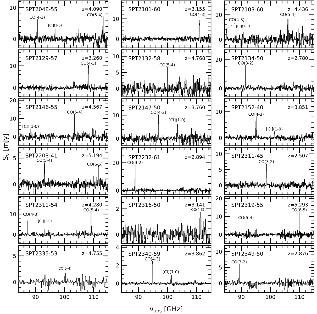
Figure B.4. (Continued) The 3mm ALMA spectra (spanning 84.2 – 114.9 GHz) of all SPT DSFGs. Marginal detections ( >3\sigma ) are designated by the smaller font and dashed line. A tentative line in SPT2340-59 was identified in Strandet et al. (2016) at 94.79 GHz. When SPT2340-59 was reobserved in Cycle 7, two lines were detected, shown above.
