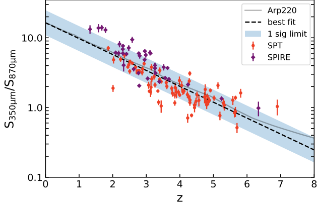
Figure 7. The S_{350\mu\text{m}}/S_{870\mu\text{m}} color serves as a rough indicator for redshift. The SPT catalog is compared to Herschel /SPIRE sources and is well-described by an exponential fit with a term to describe the intrinsic scatter. The Arp220 colors were obtained by artificially observing the Arp220 SED (Silva et al. 1998) for a range of redshifts.
