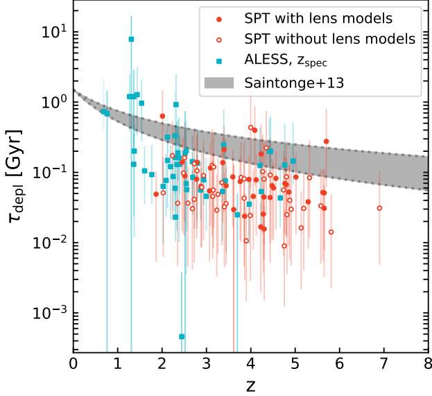
Figure 13. Depletion time ( \tau_{\text{depl}} ) versus redshift for the SPT-selected sample and ALESS sample. The extreme properties of the SPT sample result in short depletion times, which imply that the SPT sources are experiencing a rapid burst of star formation. The typical values presented in Saintonge et al. (2013) for main sequence galaxies are shown in grey.
