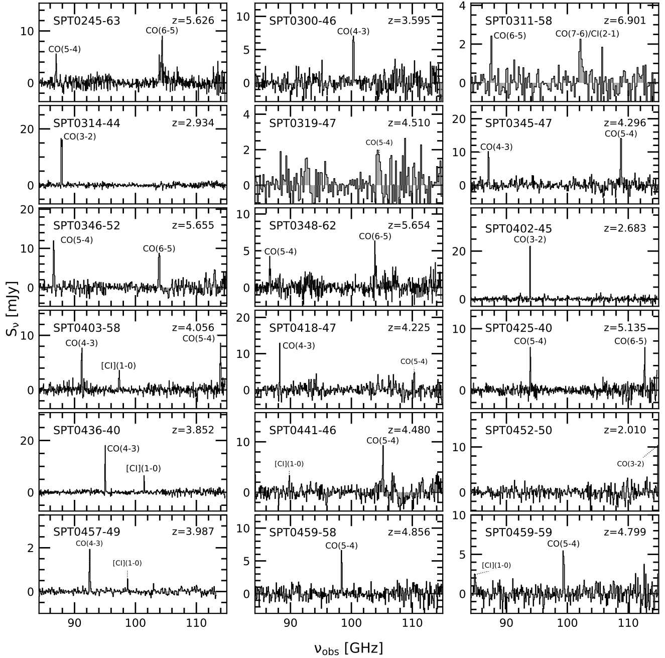
Figure B.2. (Continued) The 3mm ALMA spectra (spanning 84.2–114.9 GHz) of all SPT DSFGs. Marginal detections ( >3\sigma ) are designated by the smaller font and dashed line. Though no spectroscopic lines were detected in SPT0457-49 initially, two lines were detected when the source was reobserved, as shown above.
