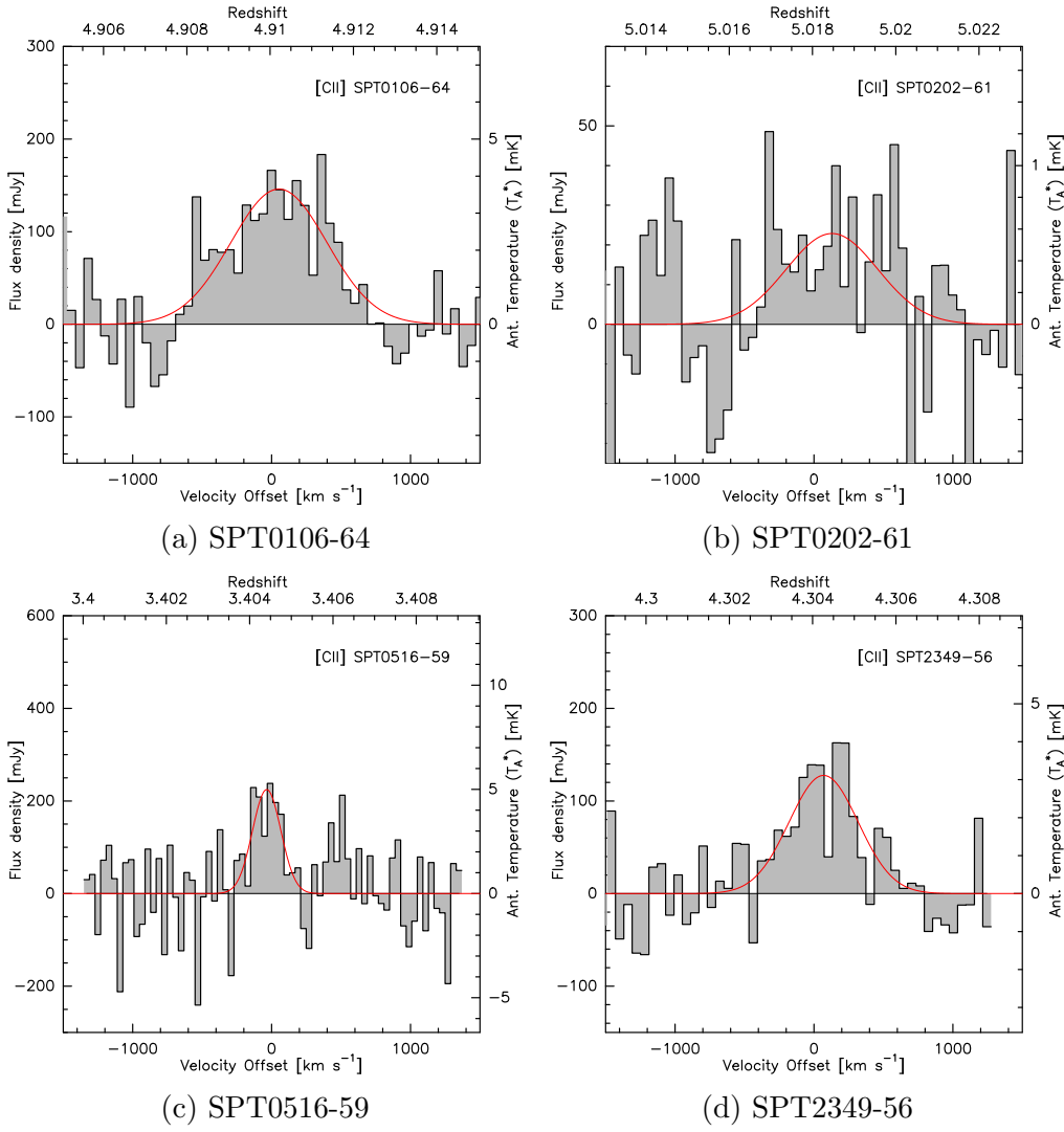
Figure C.1. APEX/FLASH [CII] redshift confirmations
