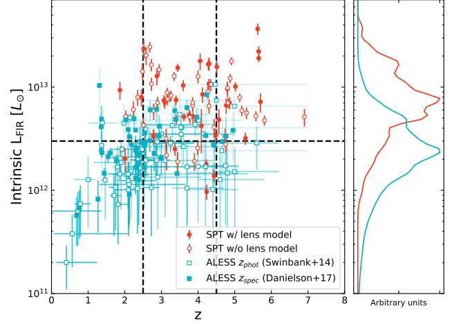
Figure 14. Intrinsic luminosity as a function of redshift for DSFGs from SPT and ALESS. SPT sources are demagnified using lens models from Spilker et al. (2016) where available. The dashed horizontal line represents the L_{\text{FIR}} above which the SPT and ALESS samples are complete, while the vertical lines correspond to 2.5 < z < 4.5 , where the surveys have equal source density.
