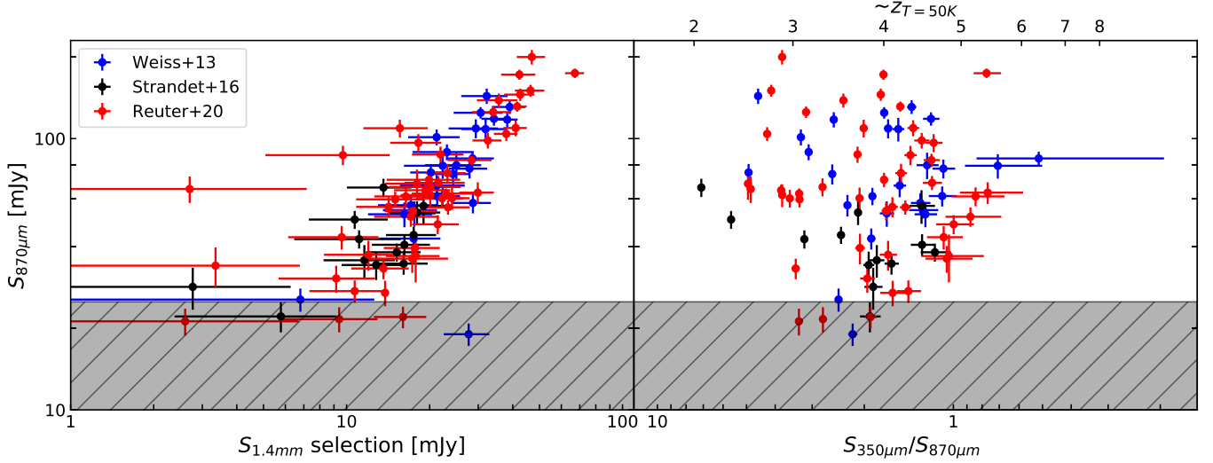
Figure 1. Flux density and color plots for all sources in the SPT-selected DSFG catalog, with 26 sources from Weiß et al. (2013) ( blue ), 15 sources from Strandet et al. (2016) ( black ) and the remaining 40 sources from this work ( red ). All of the source names and positions are detailed in Ap. A. Left: APEX/LABOCA 870\ \mu\text{m} flux density versus the SPT 1.4 mm flux selection. The initial selection included sources with a signal-to-noise ratio of 4.5, and were followed up with LABOCA. The sample is defined such that sources have S_{870\ \mu\text{m}} > 25\ \text{mJy} , excluding the grey hatched region. Sources below the S_{870\ \mu\text{m}} flux selection were not retained in the final sample. Right: The APEX/LABOCA 870\ \mu\text{m} flux density versus the ratio of the Herschel /SPIRE 350\ \mu\text{m} flux density to APEX/LABOCA 870\ \mu\text{m} flux density. The S_{350\ \mu\text{m}}/S_{870\ \mu\text{m}} color corresponds to T_{\text{dust}}/(1+z) . At a fixed T_{\text{dust}} , this color can be used as a crude proxy for redshift.
