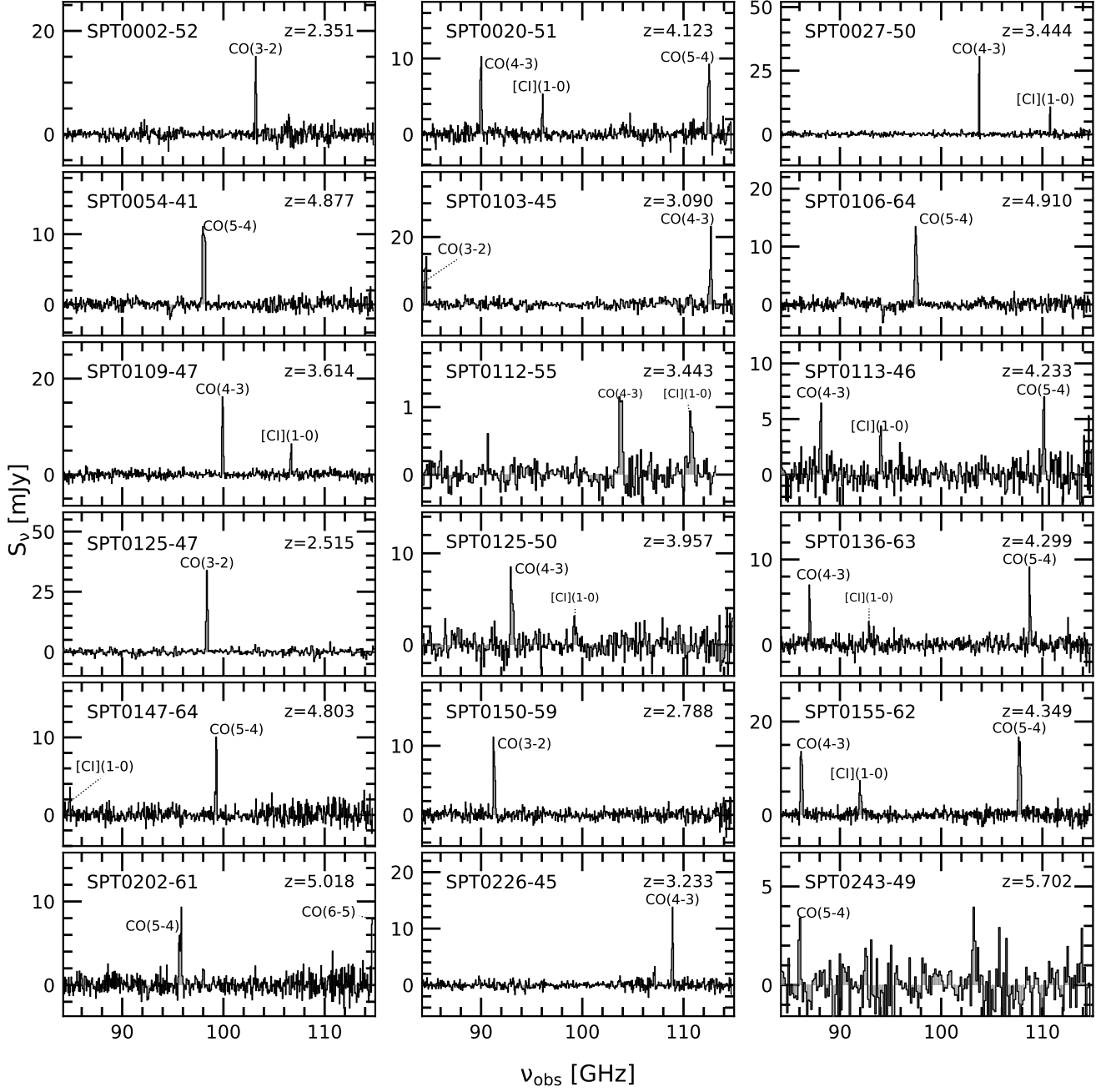
Figure B.1. The 3 mm ALMA spectra (spanning 84.2–114.9 GHz) of all SPT DSFGs. Marginal spectroscopic detections ( >3\sigma ) are designated by the smaller font and dashed line. Though no spectroscopic lines were detected in SPT0112-55 initially, two lines were detected when the source was reobserved, as shown above.
