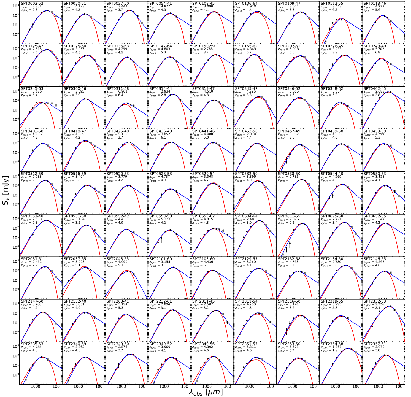
Figure 4. Spectral energy distribution fits for all 81 of the SPT-selected DSFGs. The modified blackbody model ( red ) was fit by masking data shortward of \lambda_{\text{rest}} < 50 \mu\text{m} , such that all sources have roughly uniform photometric coverage and excess emission on the Wein side of the blackbody does not artificially drive the dust temperature towards higher values. Sources which exhibit multiple components in 3 mm are fitted by masking the 3 mm point. Any photometry points which were masked for the modified blackbody fit are represented by the grey squares. In order to account for the mid-IR excess, a power law can be added on to the modified blackbody function (Blain et al. 2003) to better describe all available data ( blue ).
