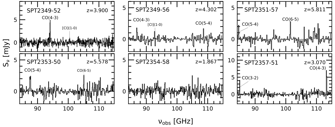
Figure B.5. (Continued) The 3mm ALMA spectra (spanning 84.2 – 114.9 GHz) of all SPT DSFGs. Marginal detections ( >3\sigma ) are designated by the smaller font and dashed line. No spectroscopic lines were detected in SPT2354-58 because it falls into a spectroscopic redshift desert, depicted in Fig. 2.
