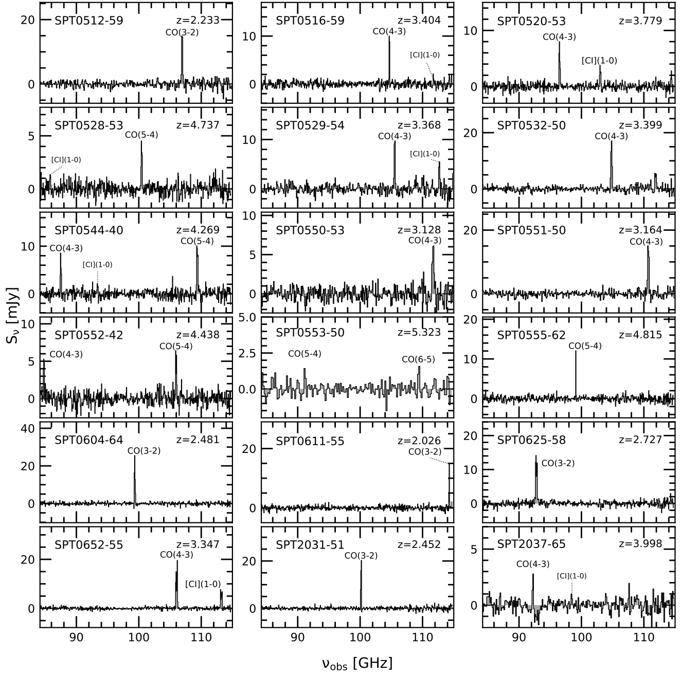
Figure B.3. (Continued) The 3mm ALMA spectra (spanning 84.2–114.9 GHz) of all SPT DSFGs. Marginal detections ( >3\sigma ) are designated by the smaller font and dashed line.
