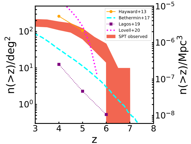
Figure 16. Spatial densities of high-redshift luminous galaxies with L_{\text{FIR}} > 3 \times 10^{12} L_{\odot} measured in this work from the SPT survey compared to model predictions from Hayward et al. (2013); B  thermin et al. (2017); Lagos et al. (2019) and Lovell et al. (2020).
