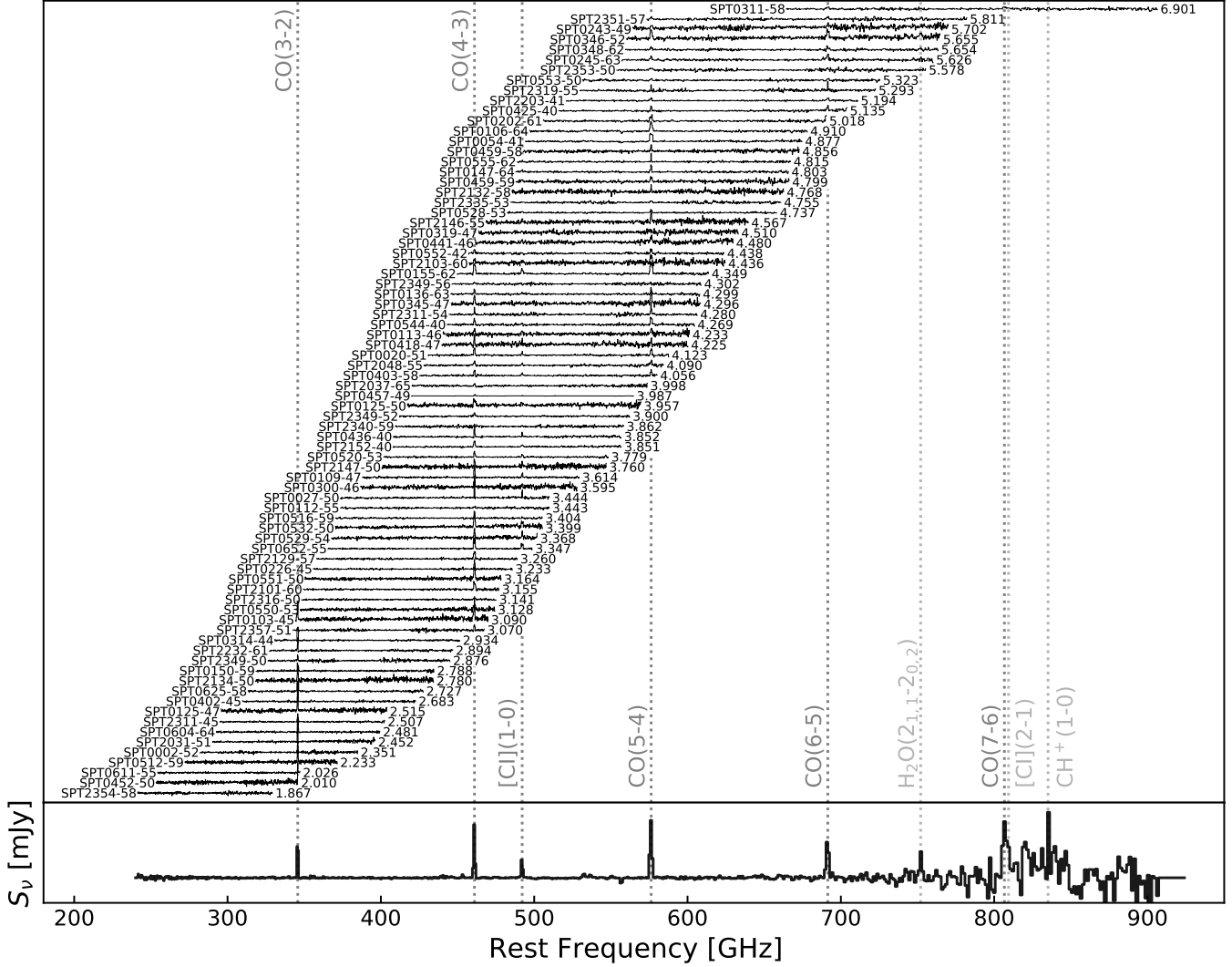
Figure 3. Top panel: All obtained ALMA 3 mm spectra in the rest frame, with channel widths of 62.5 MHz. The associated redshift is shown on the right of each spectrum. Not shown: three DSFGs which do not have ALMA 3 mm data, but were confirmed through other programs (SPT0538-50, SPT0551-48, SPT2332-53) and published in Greve et al. (2012) and Strandet et al. (2016). By performing a 1.4 mm flux-weighted average of the observed continuum-subtracted rest frame spectra, we obtain the composite spectrum presented in the bottom panel. This was first done in Spilker et al. (2014), but has been updated to include the final SPT-selected sample. Emission lines used for redshift confirmation are shown in dark grey , while other important emission lines are shown in light grey .
