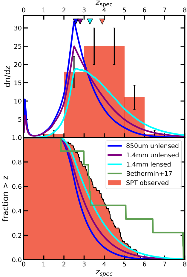
Figure 10. The observed SPT-DSFG redshift distribution is shown overlaid with modeled source catalog predictions from Béthermin et al. (2012a, 2015a) and Béthermin et al. (2017). Top: The observed redshift distribution compared with modeled source catalogs with selections of 850\ \mu\text{m} ( blue ), 1.4\ \text{mm} ( purple ) and 1.4\ \text{mm} with gravitational lensing taken into account ( cyan ). The filled triangles at the top of the panel represent the median redshifts of their respective samples. Bottom: The cumulative source density as a function of redshift.
