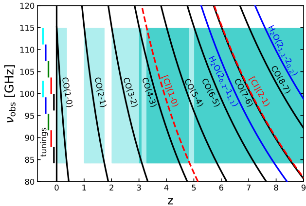
Figure 2. Spectral coverage of the important CO, [CII], and H 2 O emission lines as a function of redshift. The darker teal shaded region designates the redshift range in which two or more strong lines are expected to be detected, which would provide an unambiguous redshift for a given observation. The lighter teal region marks redshift range where only a single line is detectable, and an ancillary spectroscopic observation or photometric redshift would be required to identify the correct redshift. The five frequency tunings used in the 3 mm line scans are shown in the left panel
