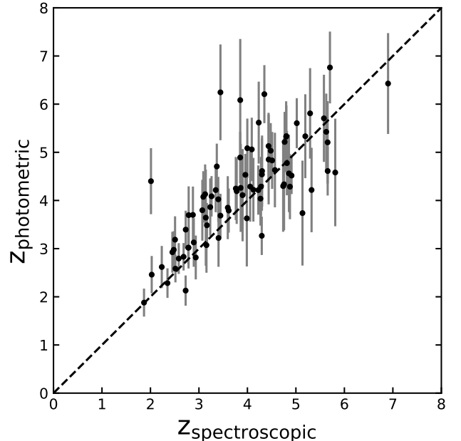
Figure 6. Photometric redshift compared with spectroscopic redshift. We find good agreement between photometric and spectroscopic redshifts, though photometric redshift has large associated errors. Unity is shown as the dashed line.
