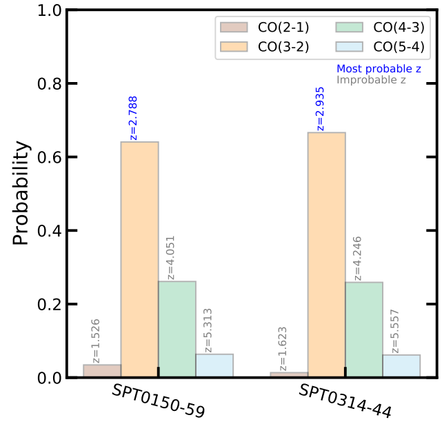
Figure C.5. Histograms showing the probability of the redshift options for each source with a single line detection in the ALMA 3 mm spectrum based on the dust temperature distribution shown in Fig. 5. The sources are sorted by most probable redshift. The bars represent the probability of each line identification, and the most probable redshift values are denoted in blue.
