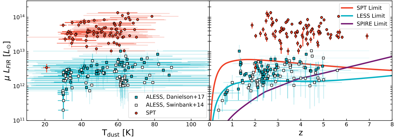
Figure 8. Left: Apparent L_{\text{FIR}} vs. T_{\text{dust}} for the unlensed ALESS sources ( teal ) presented in Swinbank et al. (2014); Danielson et al. (2017) and the lensed SPT sources presented in this work ( red ). The offset in apparent L_{\text{FIR}} between the lensed (SPT) and unlensed (ALESS) sources is due to gravitational magnification. It should be noted that for many of the ALESS sources, the photometry is not well constrained, which is reflected in the size of the associated error bars. Right: The FIR luminosity as a function of redshift for the same sources. The teal, purple, and red curves represent the limiting FIR luminosity as a function of redshift corresponding to: 3\times the LESS limit (r.m.s. \sim 1 mJy), 3\times the SPIRE 500\ \mu\text{m} confusion limit (30 mJy), and the 3\sigma SPT 2.0 mm survey limit (3.9 mJy), given the SED model of this paper and assuming a 35 K dust temperature. Many of the sources discovered in the LESS survey split into multiple components, and were treated as individual sources in the ALESS survey and consequently fall below the plotted LESS survey limit. The SPT survey, with its longer wavelength selection, is more sensitive to sources at the highest redshifts ( z > 5 ) than Herschel .
