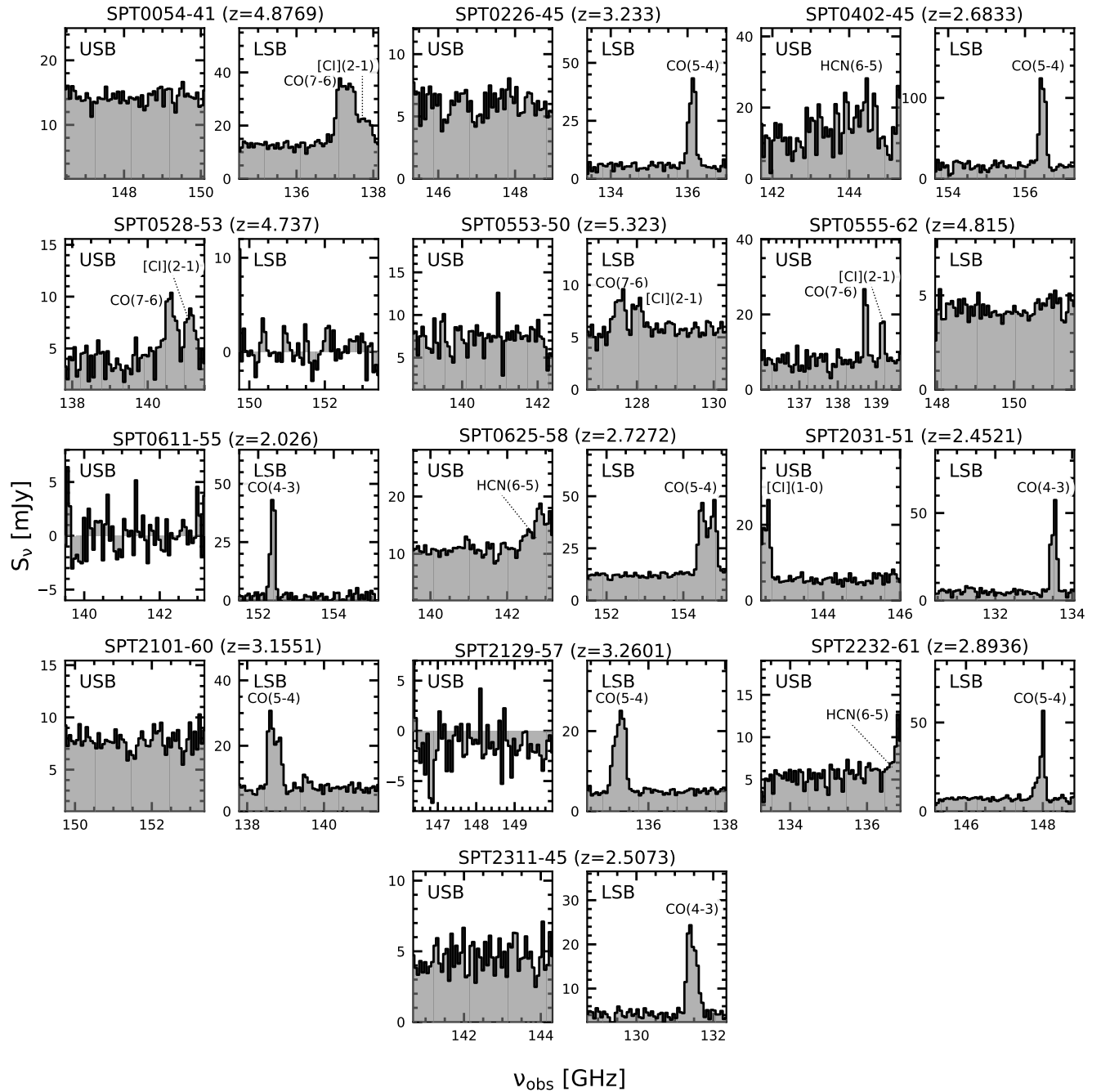
Figure C.2. ALMA 2 mm spectra for sources with redshifts based on a single 3 mm emission line. For each source we show the USB and LSB spectra in the left and right panel, respectively. Each sideband has a total bandwidth of 3.75 GHz.
