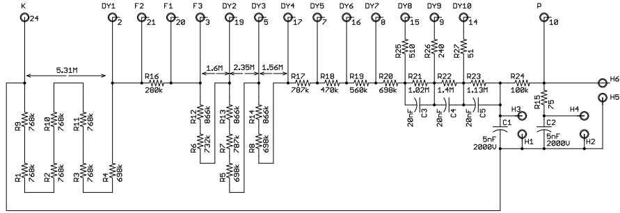
Figure 2: Circuit diagram for the PMT bases. The dynode voltages are divided in a tapered manner, and the anode has a 75 \Omega terminating resistor to minimize reflections. The labels in the figure denote: K - cathode, DYn - dynodes, Fn - focusing electrodes, P - anode, and Hn - solder pads on circuit board.
