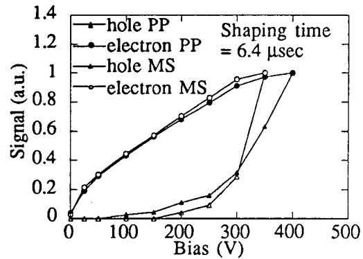
Fig.10 Charge collection in the 28 \mu\text{m} pin diodes with the parallel plate electrodes (PP) and the microstrip electrodes (MS).
