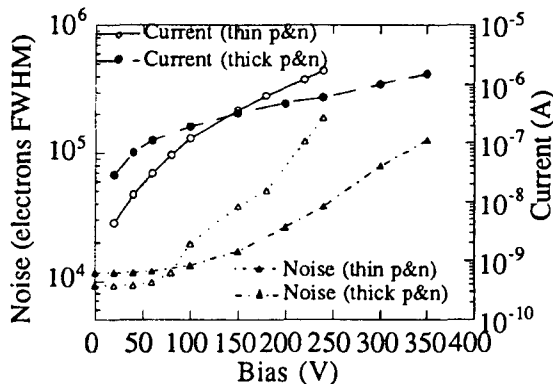
Fig.5 Noise and current-bias characteristics of a 8.7 µm diodes with thin doped layers and thick doped layers.
