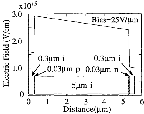
Fig.1 Calculated field profile of the 5.7 \mu\text{m} buried p-i-n diode described in the text.
