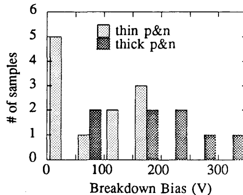
Fig.6 Breakdown bias for 8.7 µm diodes with thin and thick doped layers
