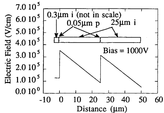
Fig.6 Calculated field profile for a diode with thin p layers buried in the thick i layer. The same charge densities are assumed as in Fig.5
