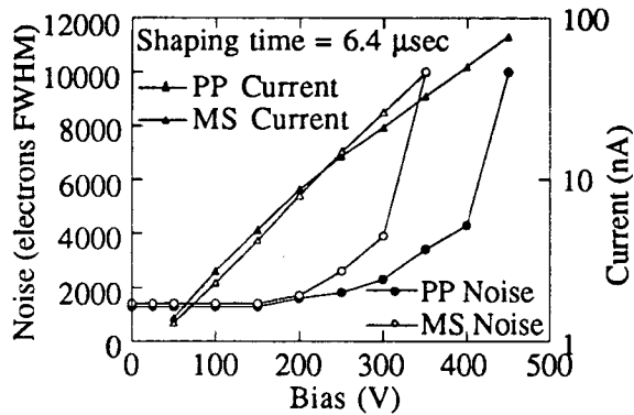
Fig.9 Noise and current-bias characteristics of 28 \mu\text{m} pin diodes with the parallel plate electrodes (PP) and the microstrip electrodes (MS).
