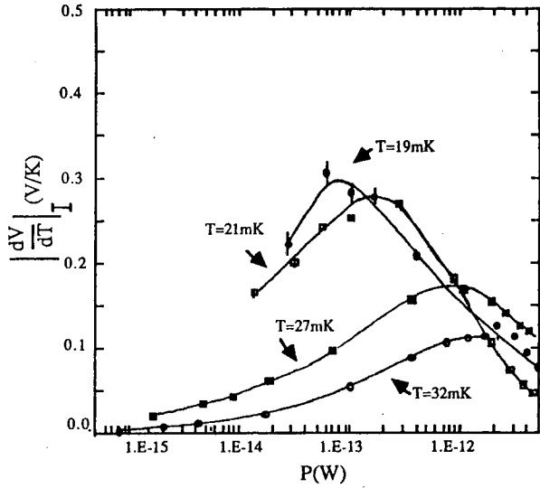
Figure 6. Responsivity |dV/dT|_1 vs. power ( P=IV ) of NTD Ge at different mixing chamber temperatures.
