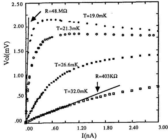
Figure 3. I-V curves of NTD Ge at different mixing chamber temperatures.
