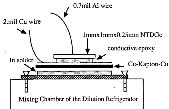
Figure 1. Installation of the thermistor on the mixing chamber of a dilution refrigerator.
