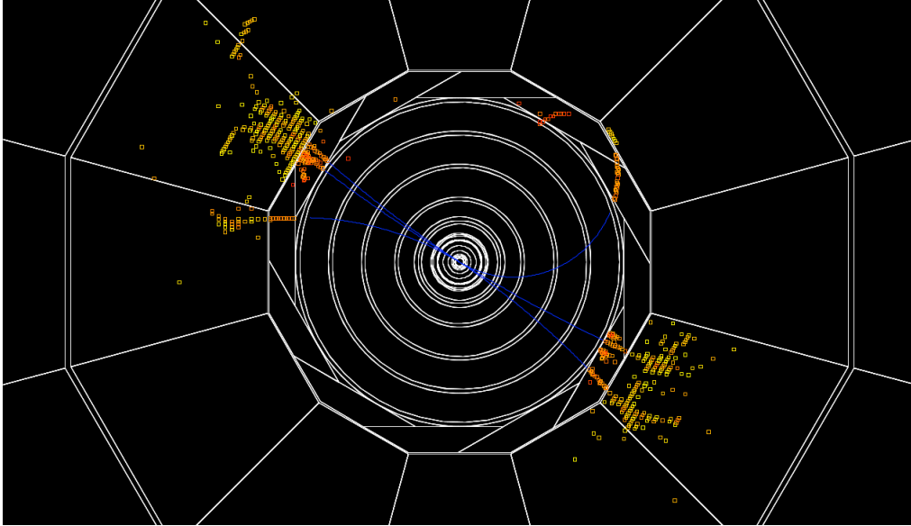
Figure 9: Wired display of a h \rightarrow \tau^+\tau^- event in the mcdrca101 detector.
