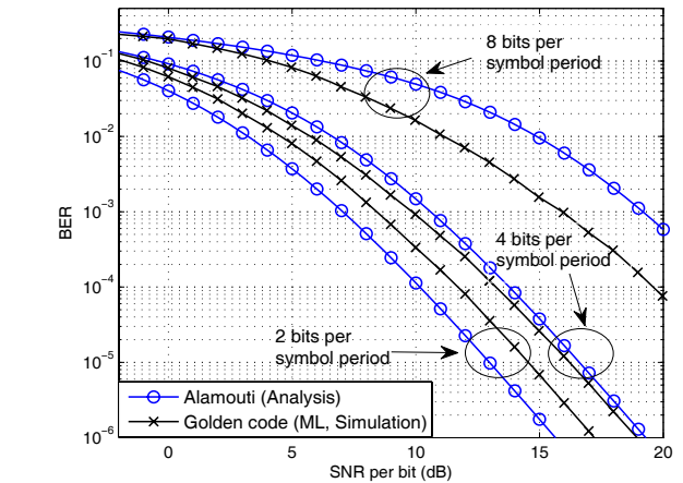
(a) Comparison of the Golden code with the Alamouti scheme
