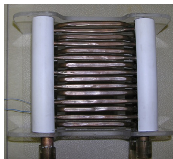
Figure 5 The thermal grill consisted of two systems of 0.75 cm-flattened copper tubing cut into approximately 10 cm in length and placed one cm apart. The inflow and outflow of the two separate systems were connected via a series of four-way valves to two separate heating and cooling water baths. The exact temperatures at the copper tubings were monitored with two separate temperature probes (Mallinckrodt Medical, Inc, St Louis, MO), which were attached to the copper tubings.
