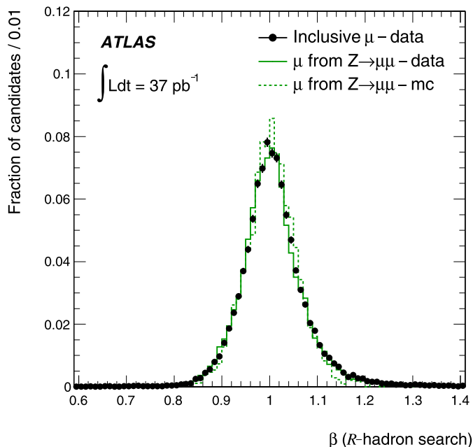
Fig. 1. Distribution of \beta for all candidates in data (points with error bars), muons from the decay Z \rightarrow \mu\mu in data (full lines) and smeared Monte Carlo (dashed lines), in the estimation used in the slepton search (upper) and in the estimation used in the R -hadron search (lower).
