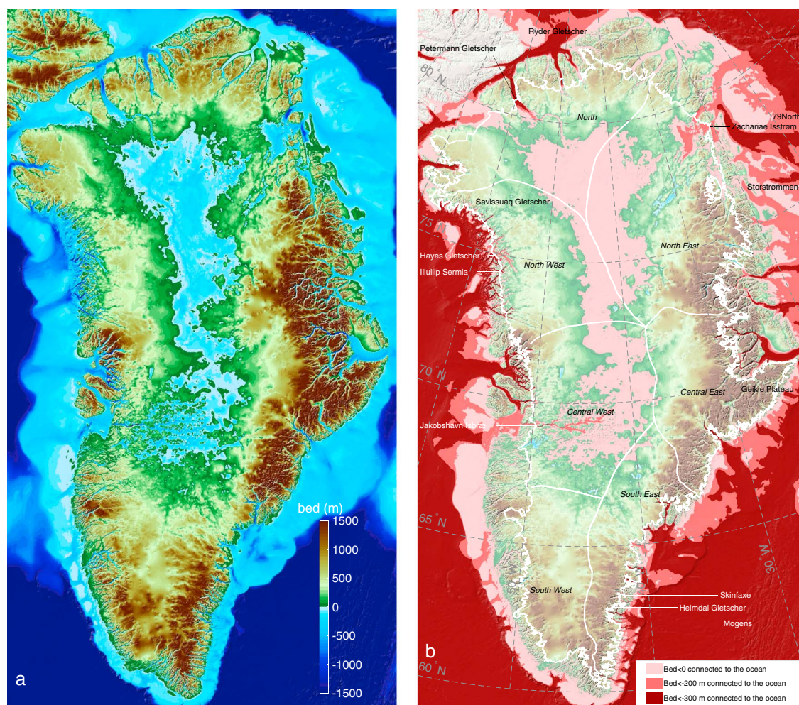
Figure 2. (a) BedMachine v3 bed topography (m), color coded between -1500 m and +1500 m with respect to mean sea level, with areas below sea level in blue and (b) regions below sea level (light pink) that are connected to the ocean and maintain a depth below 200 m (dark pink) and that are continuously deeper than 300 m below sea level (dark red). The thin white line shows the current ice sheet extent.
