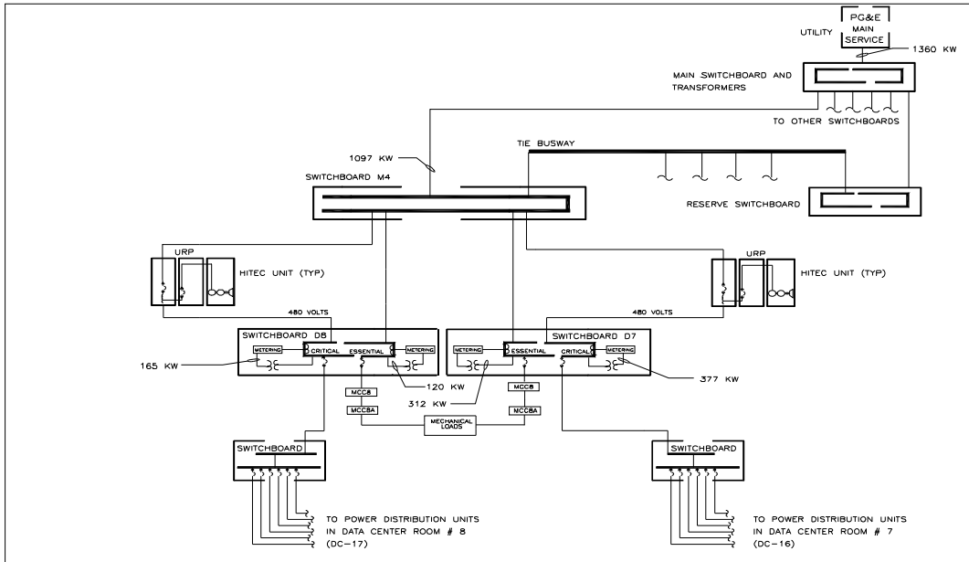
Figure 16. Electrical System Schematic
