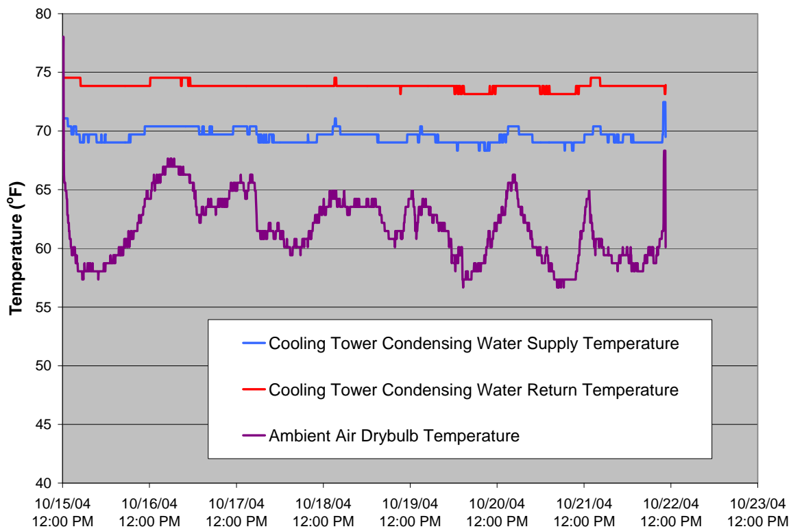
Figure 10. Cooling Tower Condenser Water Temperatures
