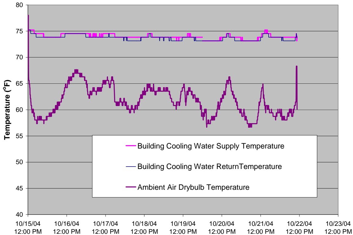
Figure 11. Secondary Condenser Water Temperatures
