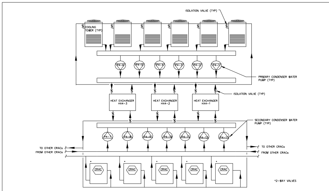
Figure 17. Condenser Water Flow Diagram
