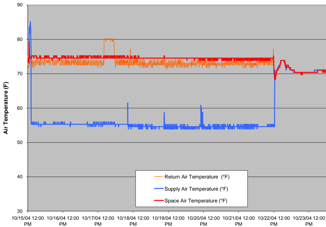
Figure 13. DC #16 CRAC 7-12 Air Temperature
