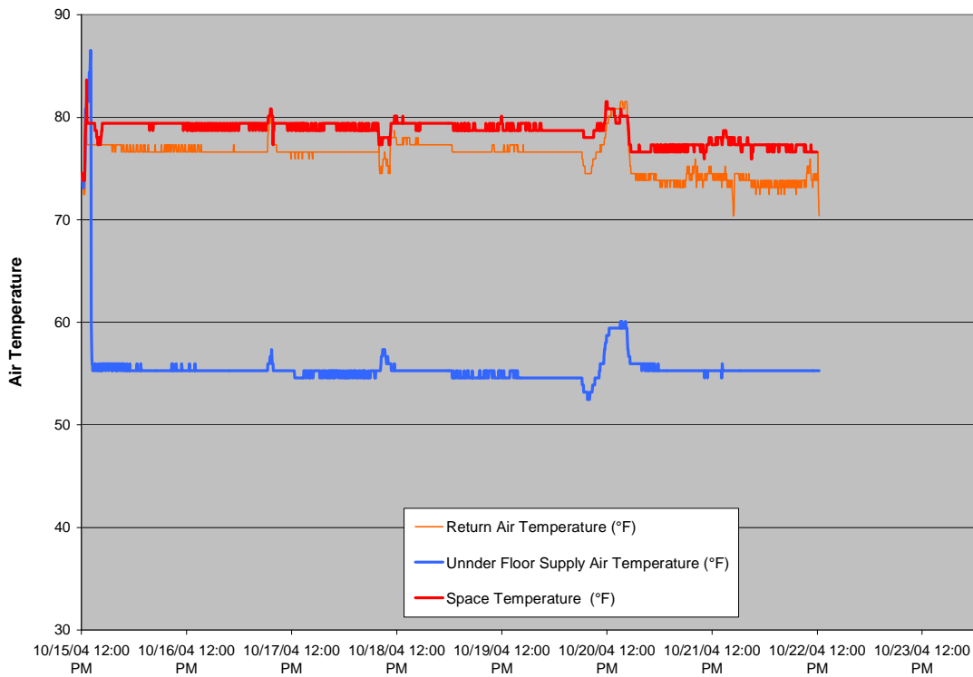
Figure 14. DC# 17 CRAC 8-3 Air Temperatures
