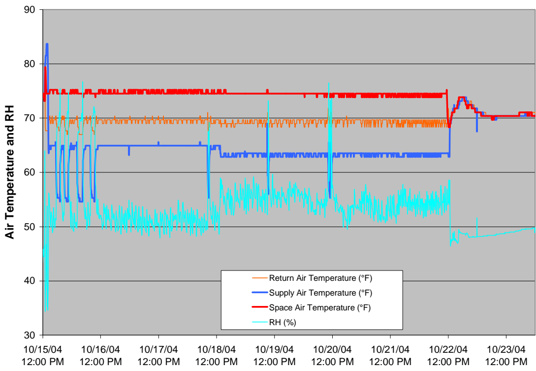
Figure 12. DC #16 CRAC 7-3 Air Temperature and Humidity
