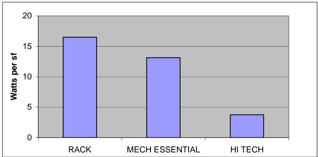
Figure 8. Data Center 17 Power Density
