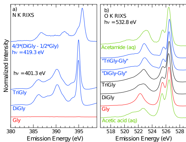
Figure 6: a) N K RIXS spectra of glycine (Gly), diglycine (DiGly), and triglycine (TriGly), excited at 401.3 eV. For comparison, the weighted difference between the non-resonant spectra of diglycine and glycine is shown at the top. b) O K RIXS spectra of glycine, diglycine, and triglycine, excited at 532.8 eV. For comparison, the spectra of aqueous solutions of acetamide (top) and acetic acid (bottom) are also shown. Above the spectrum of triglycine, weighted and magnified differences between the spectra of di-/triglycine and glycine are depicted (the weighting is discussed in detail in the text).
