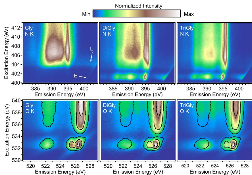
Figure 4: N K (top) and O K (bottom) RIXS maps of glycine (Gly), diglycine (DiGly), and triglycine (TriGly). The color-coded RIXS intensity is shown as a function of excitation and emission energy. For better visualization of differences in the O K RIXS maps, the map of glycine is also superimposed on the maps of diglycine and triglycine as black contour lines.
