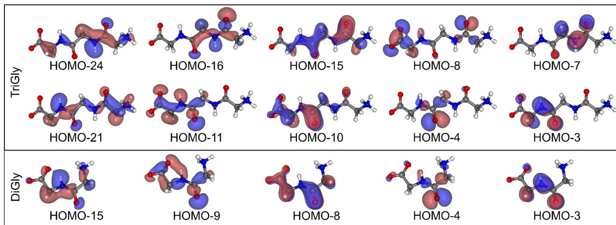
Figure 3: Molecular structure and calculated orbital iso-density surfaces of selected occupied molecular orbitals of diglycine (bottom) and triglycine (top).
