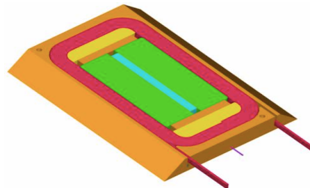
Fig. 2: Optimized HCX coil module
