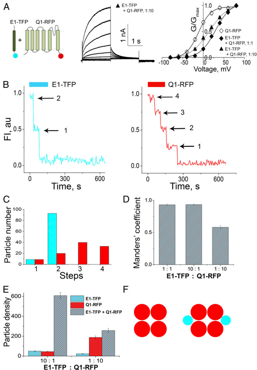
Fig. 5. Limiting amounts of E1-TFP reveal two channel types, those with two E1 subunits and those with none. E1-TFP was added at 1/10th the concentration of Q1-RFP and CHO cells studied by voltage-clamp in whole-cell mode or by TIRFM with simultaneous photobleaching of each FP. Currents were evoked and analyzed as described in Materials and Methods . Data are means \pm SEM for five cells studied in each group. Biophysical parameters are summarized in SI Appendix, Table S1 , and the analysis of bleaching steps is in SI Appendix, Table S3 . (A, Left) Cartoon of E1-TFP and Q1-RFP showing the FPs on the subunit C termini. (Center) Family of whole cell-currents from cells with 10-fold less E1-TFP than Q1-RFP showing a rapid rise in current not seen when E1 + Q1 subunits are expressed at equal levels (Fig. 1A). (Right) Normalized G - V relationships for cells expressing Q1-RFP alone (open diamond), equal E1-TFP and Q1-RFP cDNA (1:1; filled diamond), and 10-fold less E1-TFP with Q1-RFP (1:10; filled triangle). (B) Time courses for simultaneous photobleaching of both fluorophores in a representative fluorescent particle with E1-TFP and Q1-RFP. E1-TFP bleaches in two steps, and Q1-RFP bleaches in four steps (arrows). (C) Histogram of photobleaching steps for E1-TFP (teal bars) and Q1-RFP (red bars) studied in the same fluorescent spots. No colocalized particles were observed to bleach with more than two steps for E1-TFP or four steps for Q1-RFP. (D) Histograms of Manders' coefficient of colocalization from cells expressing E1-TFP with Q1-RFP at 1:1, 10:1, or 1:10 ratios ( SI Appendix, Table S4 ) showing that \sim half the particles have both E1 and Q1 subunits and half have only Q1 subunits with E1 at 1/10th the level of Q1. (E) Surface-density histogram for subunits based on bleaching steps (using Manders' coefficient of colocalization; SI Appendix, Table S4 ) for cells expressing E1-TFP with Q1-RFP at 10:1 and 1:10 ratios showing E1-TFP alone (teal bars), Q1-RFP alone (red bars), or the two subunits when colocalized (striped bar). (F) Cartoon representation of the two channel types found on the cell surface when E1 is limiting—Q1 channels with no E1 and I_{Ks} channels with two E1 subunits.
